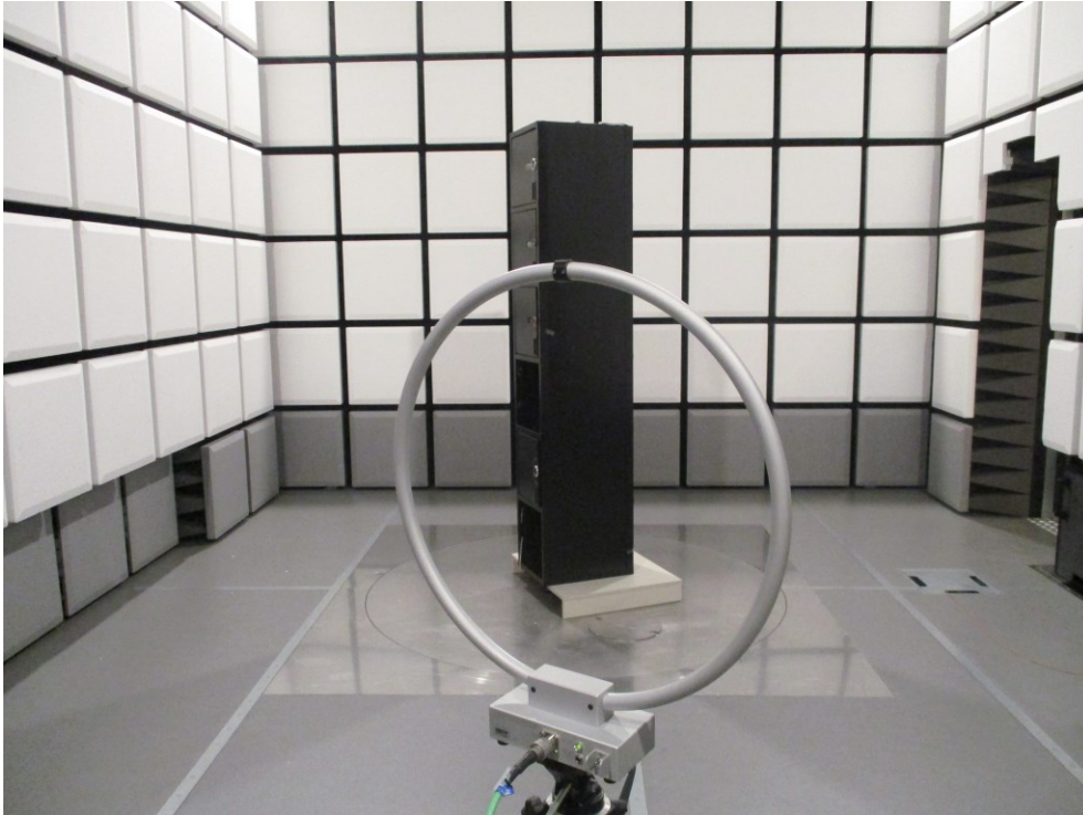
Figure 2: Radiated emission test from 9 kHz to 30 MHz
