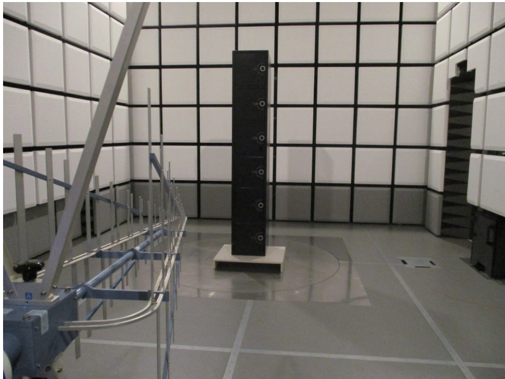
Figure 4: Radiated emission test from 200 MHz to 1 GHz
