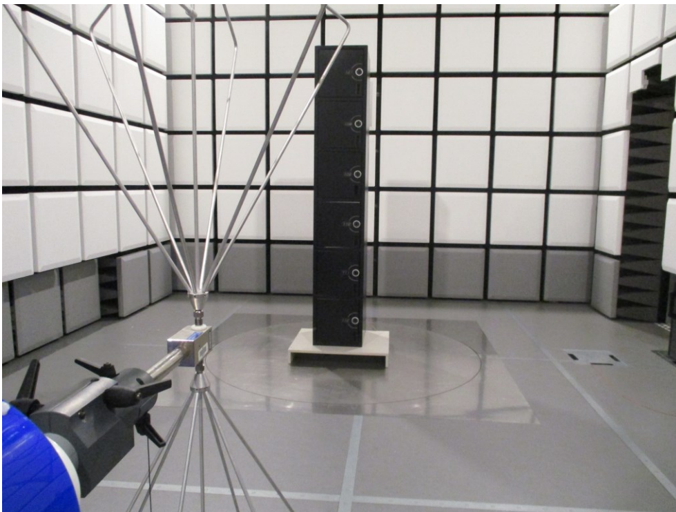
Figure 3: Radiated emission test from 30 MHz to 200 MHz
