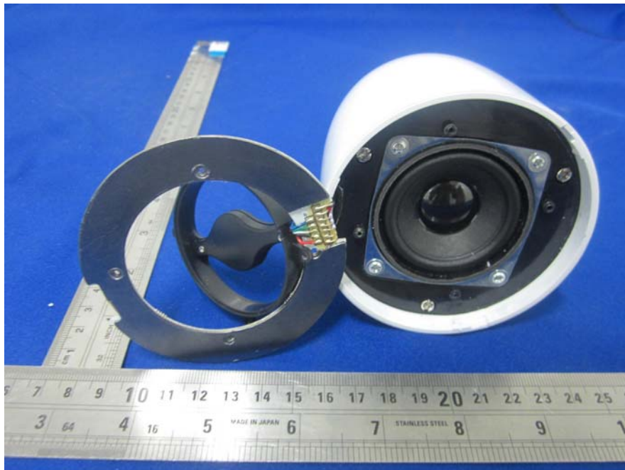
EUT –Lamp Board Off View
