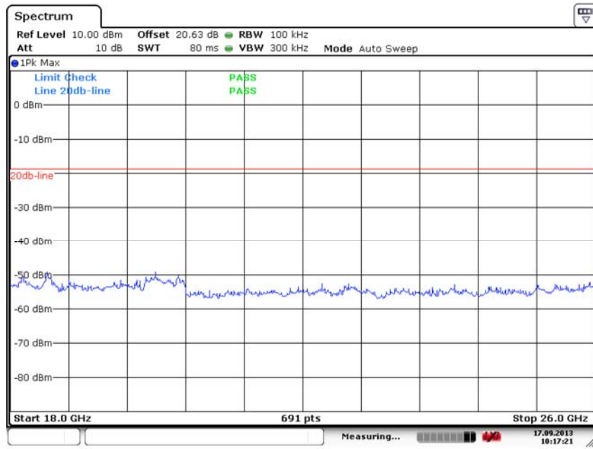
Fig. 21 Conducted Spurious Emission (All channels, 18 GHz-26 GHz)
