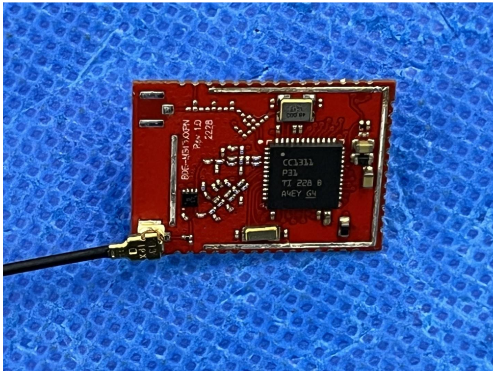
Series Model: BDE-SG1311P3N OPEN VIEW OF EUT(FIGURE 1)
