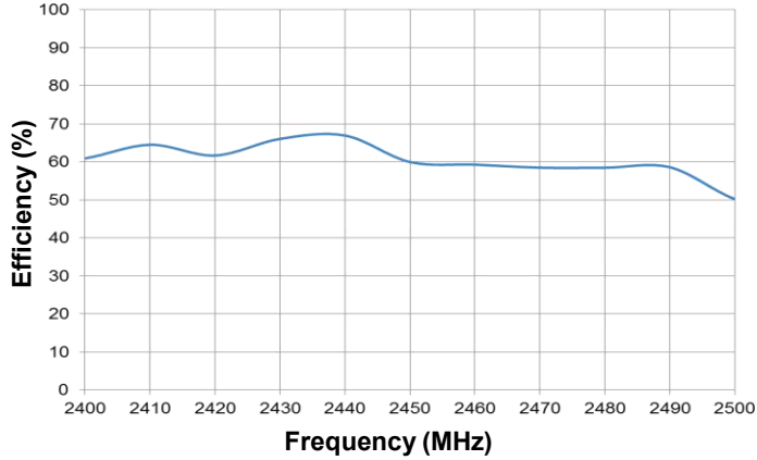
2.4 GHz Efficiency
