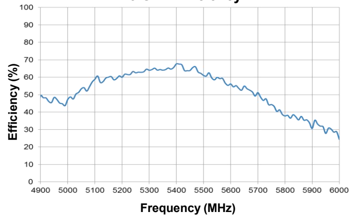
5 GHz Efficiency
