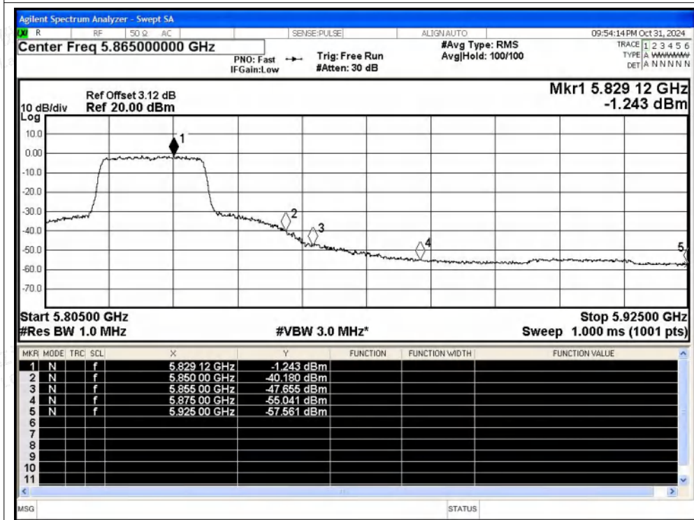
Restrict Band NVNT ax20 5825MHz Ant1 Average
