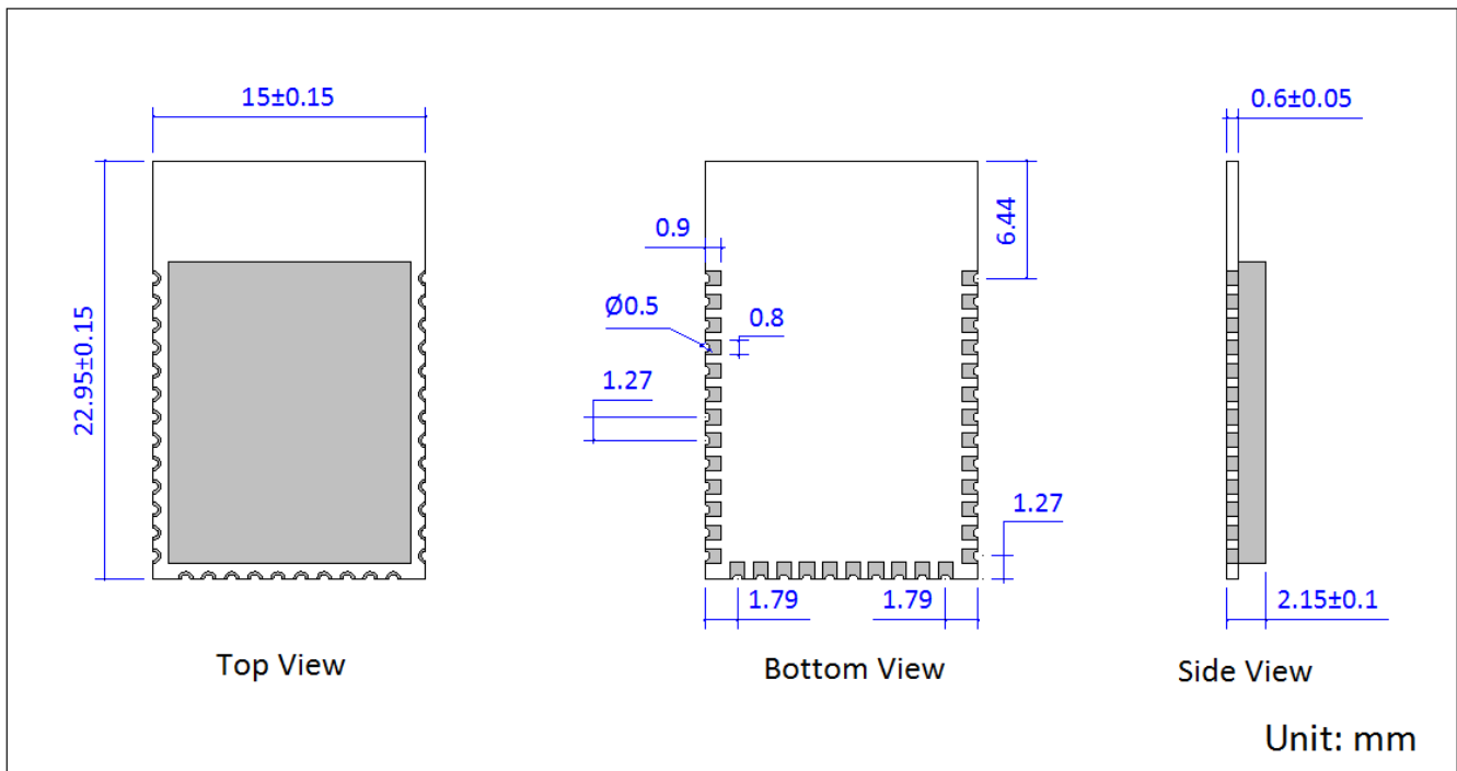
Fig. 3: Overall Dimensions of BDE-BLEM205-IN
