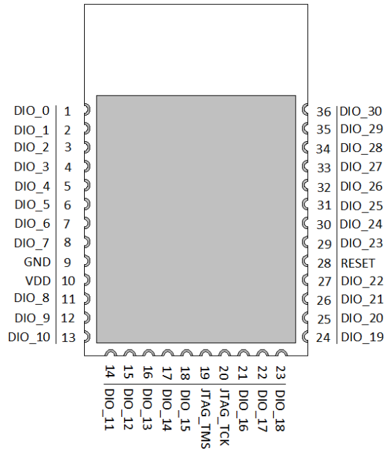
Fig. 2: The pinout of BDE-BLEM205-IN (TOP VIEW)
