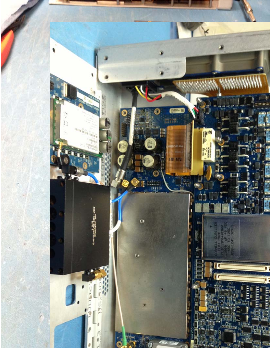
Figure 10: MCIM Top View Circuitry
