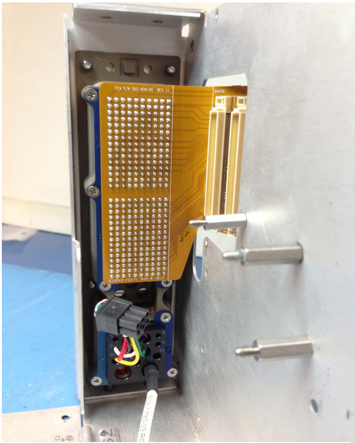
Figure 34: Rear Connector
