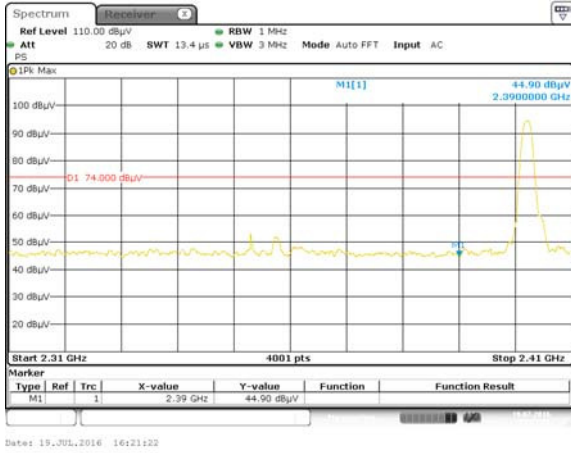
GFSK LOW CHANNEL , PEAK
