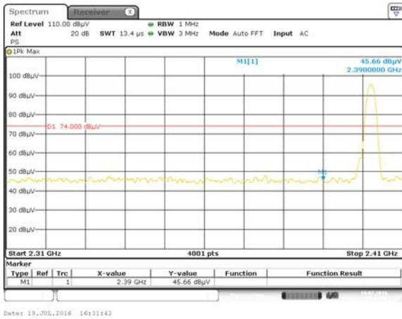
8-DPSK LOW CHANNEL , PEAK
