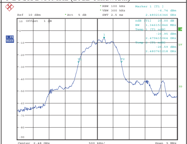
8-DPSK 2480MHz (20dB bandwidth)
