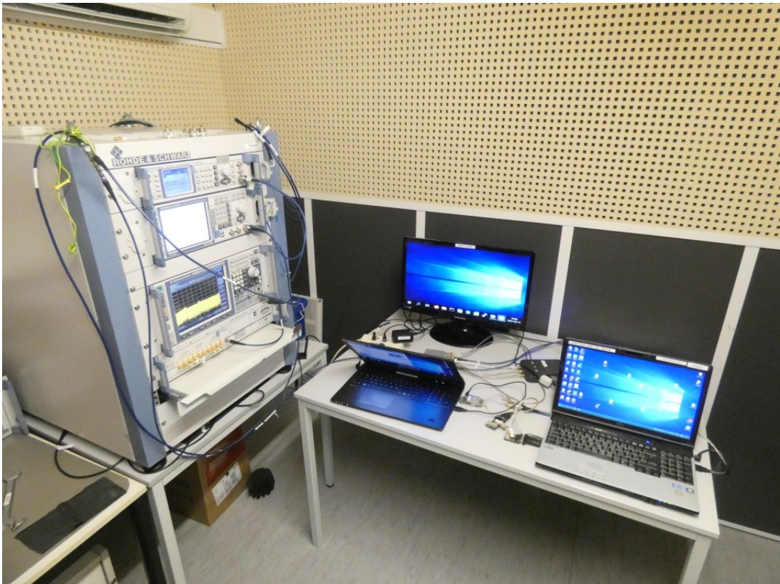
Photo 1: Test setup for conducted DFS measurements
