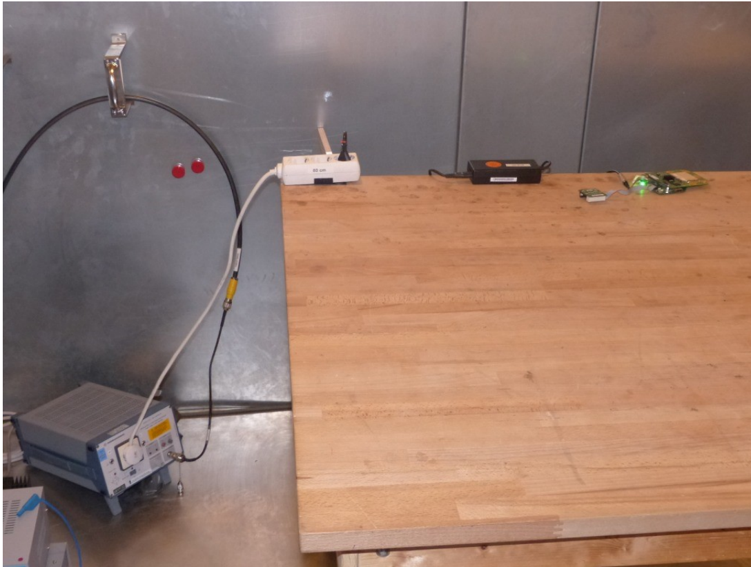
Photo 6: Test setup for conducted measurements (AC Mains)
