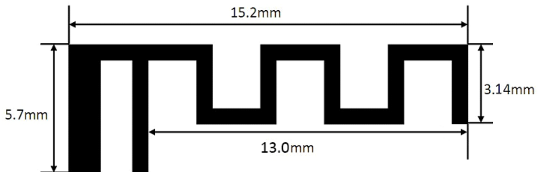
Antenna Photo & Length (mm) PCB antenna
