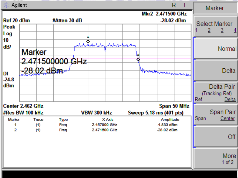
Channel 11 (2462MHz)
