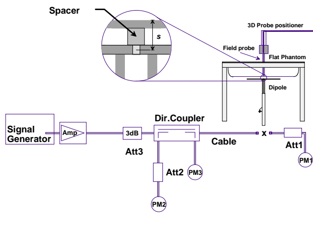
Fig 8.3.1 System Performance Check Setup
