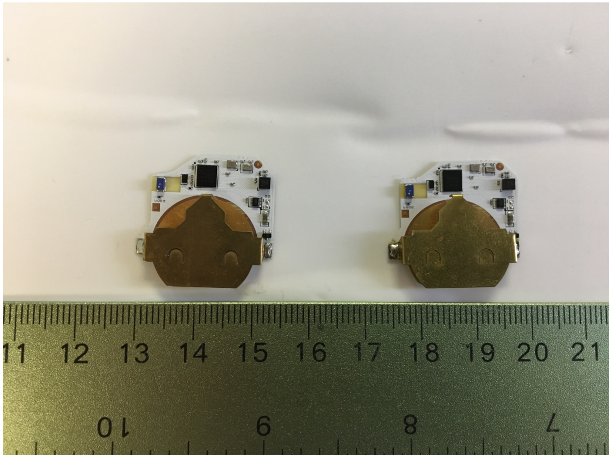
Figure 1. EUT Without Enclosure, Front (CR2020 version Left, CR2032 version Right)
