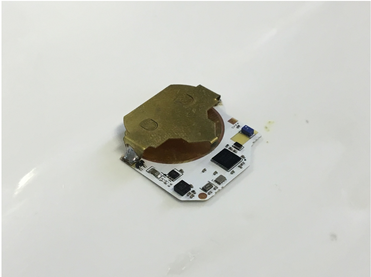
Figure 8. EUT without Enclosure, Side 2
