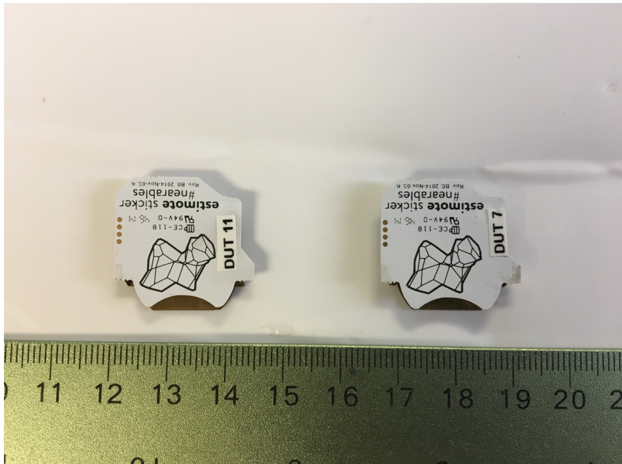
Figure 2. EUT without Enclosure, Back (CR2020 Version on Left, CR2032 Version on Right)
