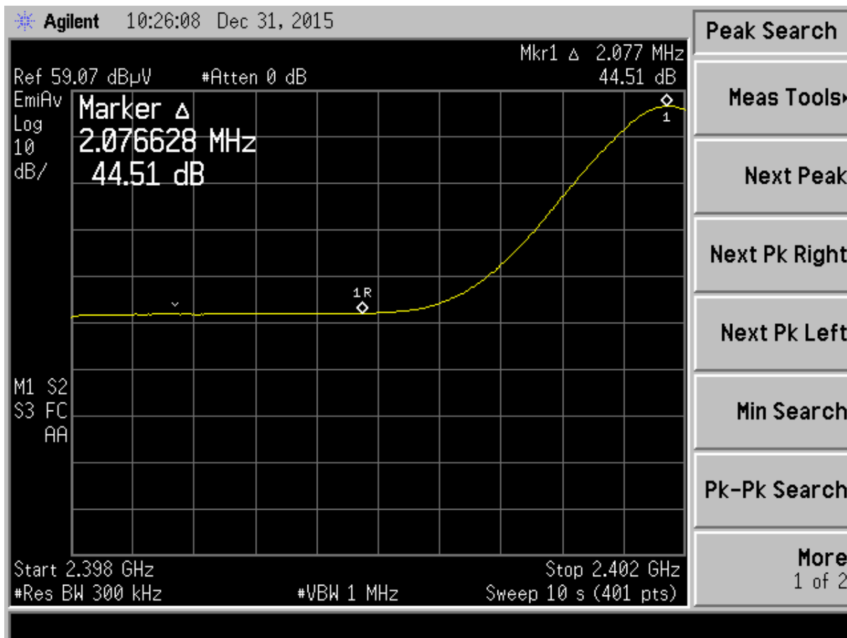
Figure 5. Band Edge Compliance, Low Channel Delta - Average
