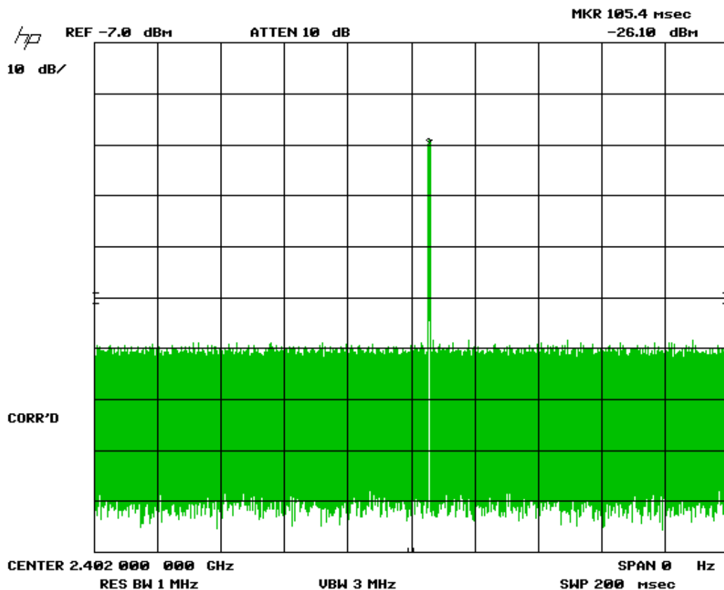
Figure 2. Duty Cycle 200ms Sweep
