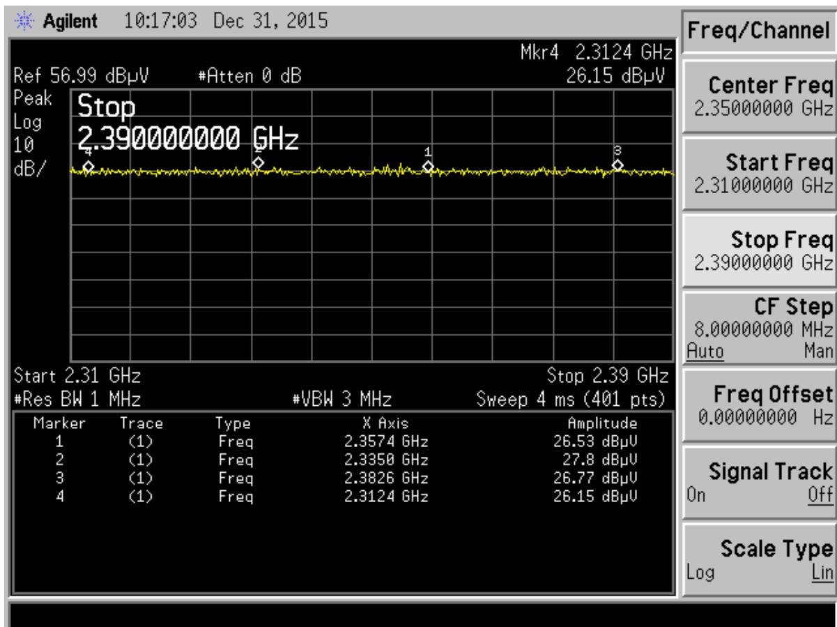
Figure 6. Radiated Restricted Band 2310 MHz to 2390 MHz, Peak
