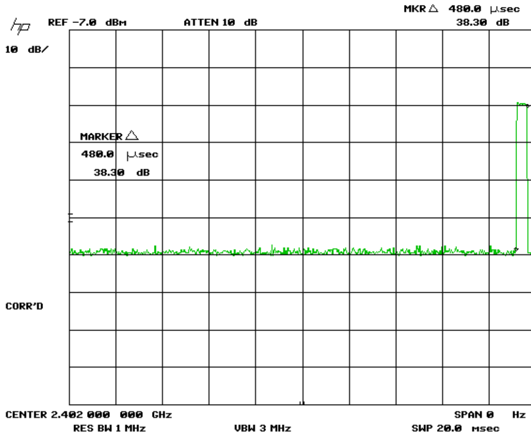
Figure 3. Transmitter Pulse Width
