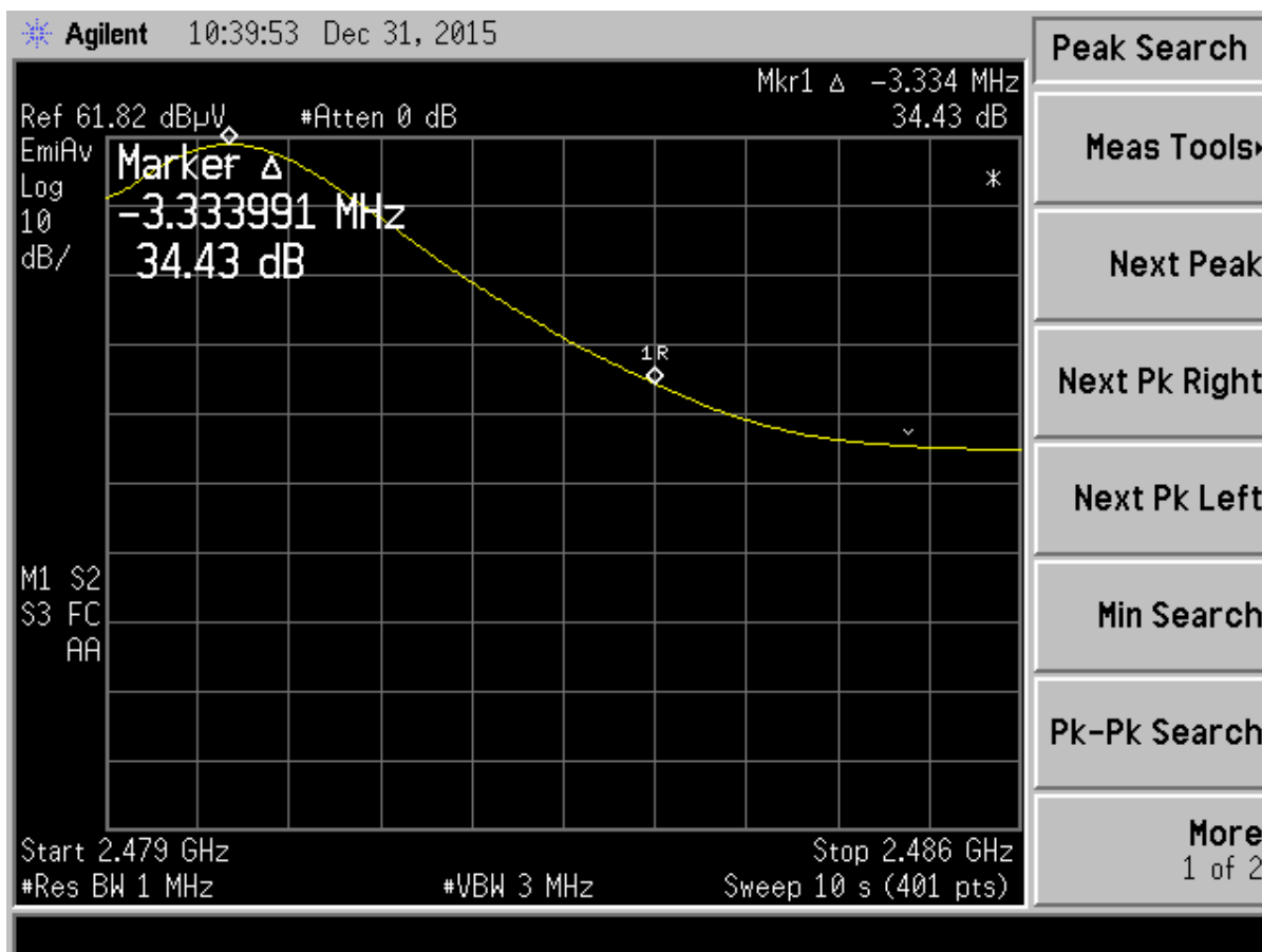
Figure 8. Band Edge Compliance, High Channel Delta – Average
