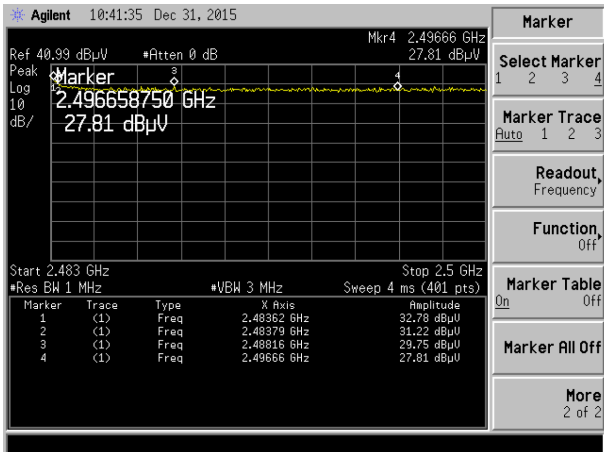
Figure 9. Radiated Restricted Band 23483.5 MHz to 2500 MHz, Peak
