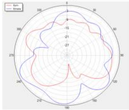
Theta=90 freq=2540MHz
