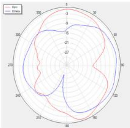
Phi=90 freq=1600MHz
