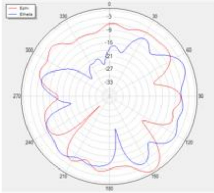
Phi=90 freq=2540MHz
