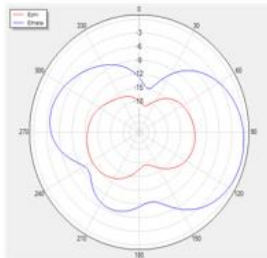
Theta=90 freq=800MHz
