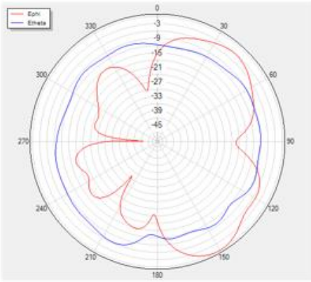
Phi=90 freq=2470MHz
