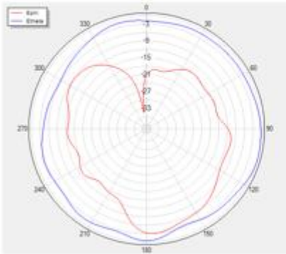
Phi=90 freq=800MHz
