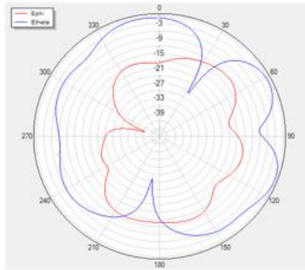
Theta=90 freq=2480MHz
