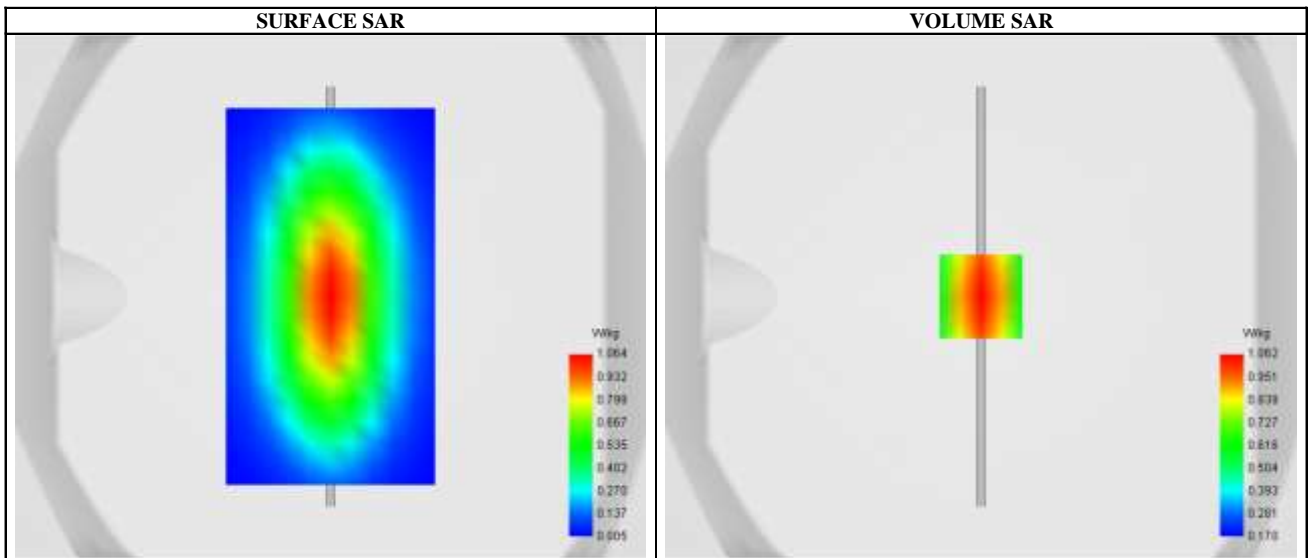
Maximum location: X=0.00, Y=0.00; SAR Peak: 1.46 W/kg
