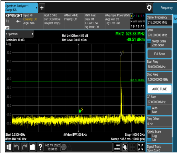
Band5-10MHz-16QAM-20525-1RB#0-Range1:30~1000MHz
