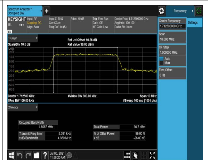
Band4-5MHz-16QAM-20375-25RB#0
