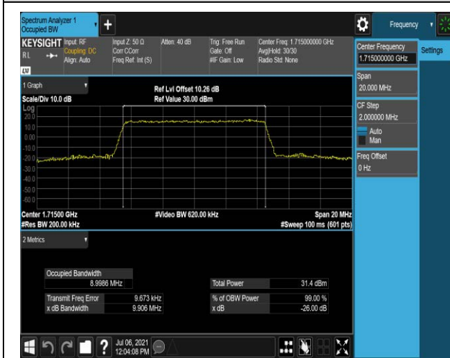
Band4-10MHz-QPSK-20350-50RB#0
