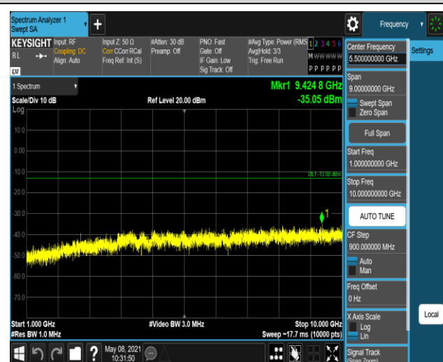
Band5-1.4MHz-QPSK-20643:1000~10000MHz
