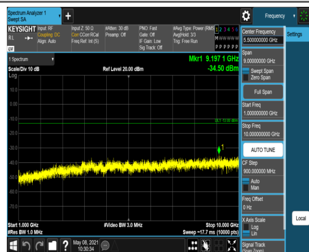
Band5-1.4MHz-QPSK-20643:1000~10000MHz
