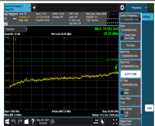
Band4-20MHz-16QAM-20175:1000~20000MHz
