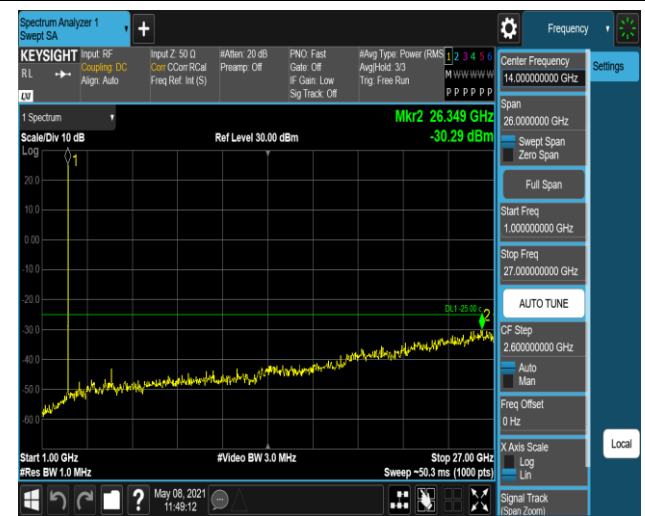
Band7-5MHz-16QAM-21100:1000~27000MHz
