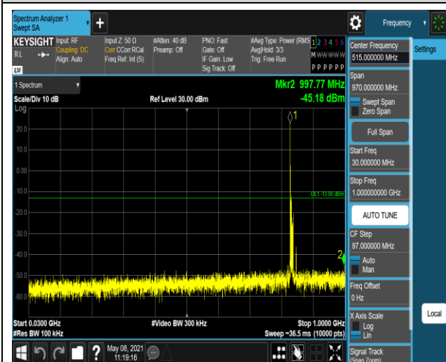
Band5-10MHz-16QAM-20600:30~1000MHz
