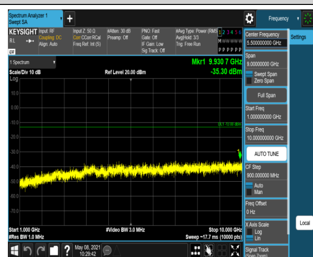
Band5-1.4MHz-16QAM-20525:1000~10000MHz
