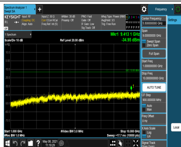
Band5-10MHz-16QAM-20600:1000~10000MHz
