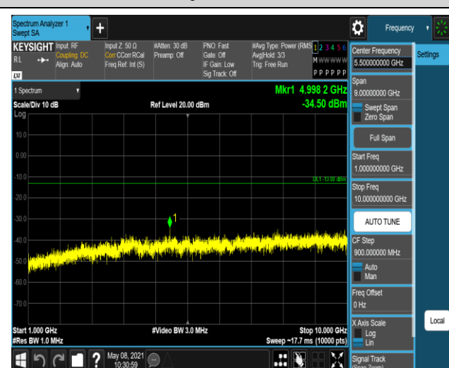
Band5-1.4MHz-16QAM-20643:1000~10000MHz
