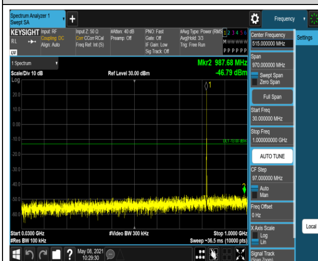
Band5-1.4MHz-16QAM-20525:30~1000MHz
