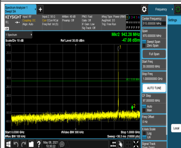
Band5-1.4MHz-QPSK-20643:30~1000MHz
