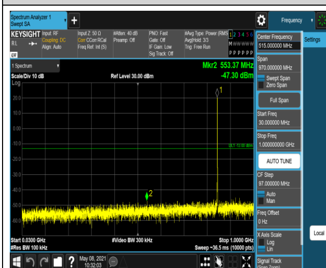
Band5-1.4MHz-16QAM-20643:30~1000MHz
