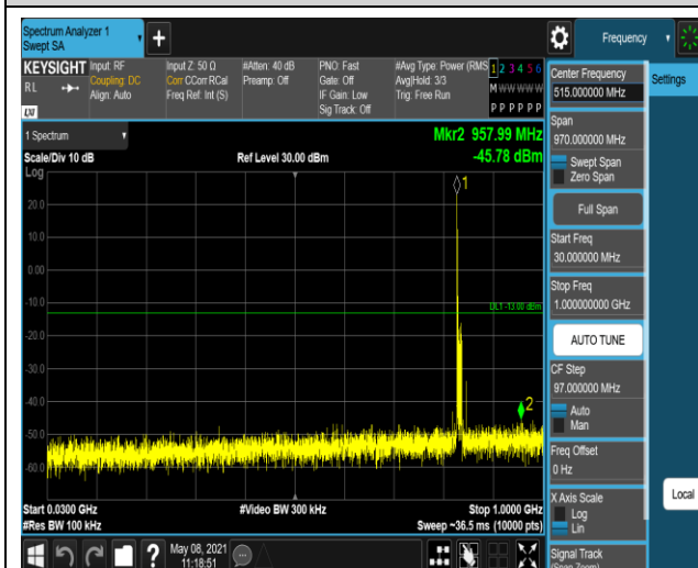
Band5-10MHz-QPSK-20600:30~1000MHz
