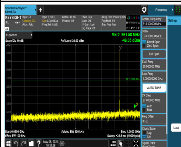
Band5-1.4MHz-QPSK-20643:30~1000MHz
