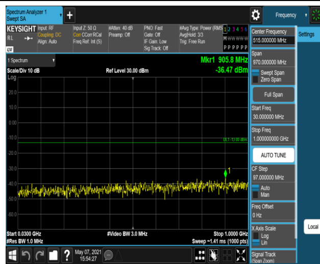
Band2-1.4MHz-QPSK-18900:30~1000MHz
