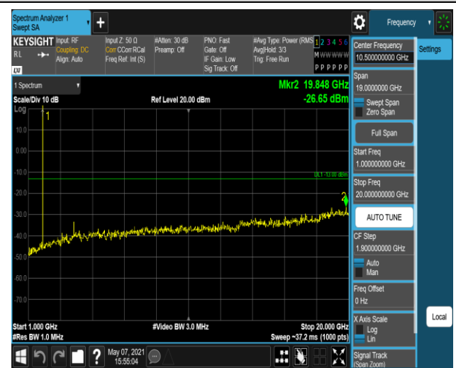
Band2-1.4MHz-16QAM-18900:1000~20000MHz
