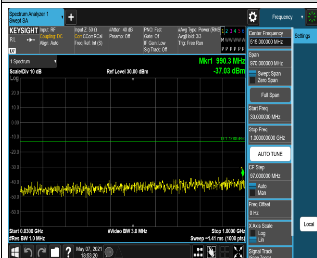
Band2-20MHz-QPSK-19100:30~1000MHz
