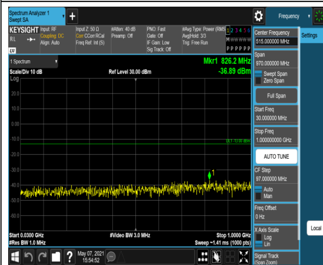
Band2-1.4MHz-16QAM-18900:30~1000MHz
