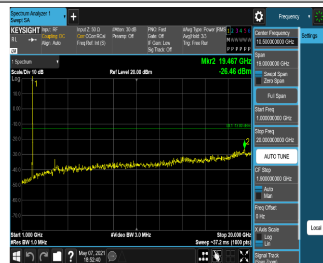
Band2-20MHz-QPSK-19100:1000~20000MHz
