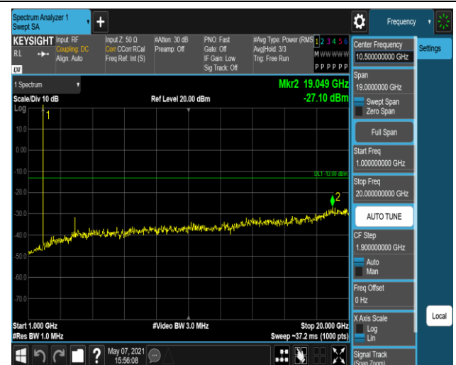
Band2-1.4MHz-16QAM-19193:1000~20000MHz
