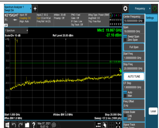
Band2-1.4MHz-16QAM-19193:1000~20000MHz
