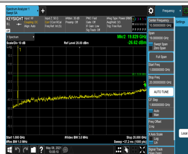
Band4-20MHz-QPSK-20300:1000~20000MHz
