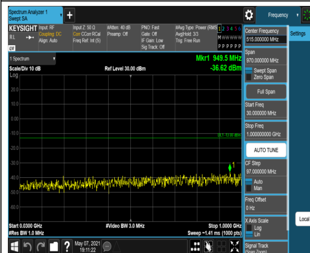
Band4-1.4MHz-16QAM-20393:30~1000MHz
