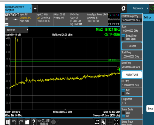
Band2-20MHz-QPSK-19100:1000~20000MHz
