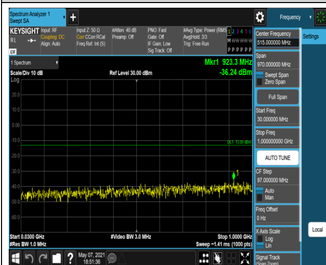
Band2-20MHz-QPSK-18900:30~1000MHz
