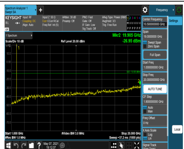
Band4-1.4MHz-16QAM-20393:1000~20000MHz
