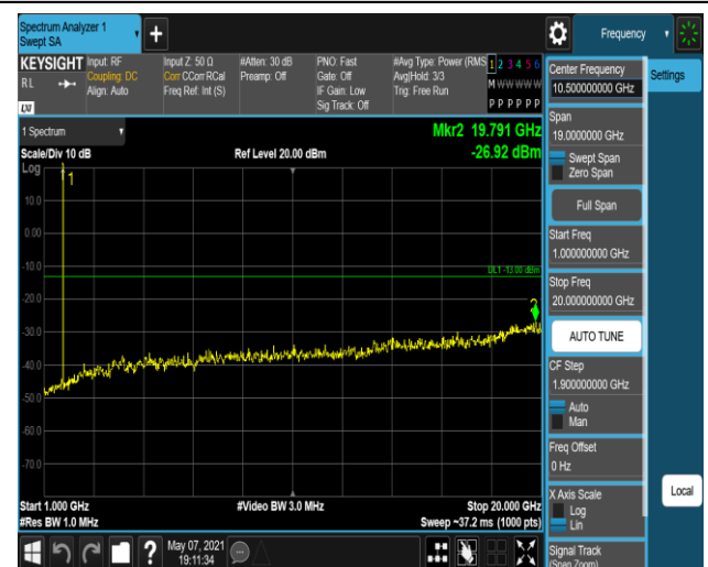
Band4-1.4MHz-16QAM-20393:1000~20000MHz
