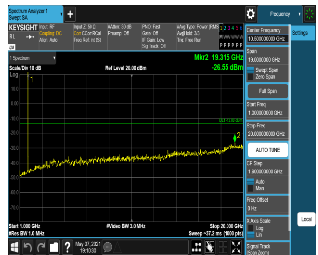
Band4-1.4MHz-16QAM-20175:1000~20000MHz
