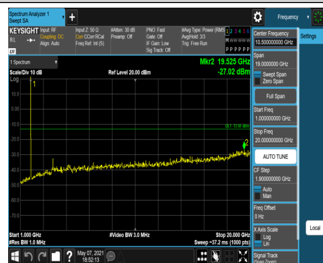
Band2-20MHz-16QAM-18900:1000~20000MHz
