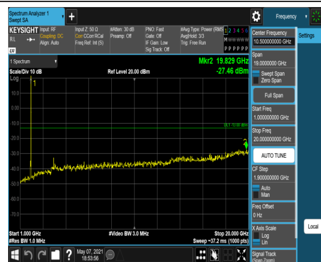
Band2-20MHz-16QAM-19100:1000~20000MHz
