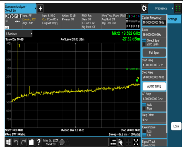
Band2-1.4MHz-QPSK-18900:1000~20000MHz
