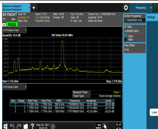
Band4-20MHz-16QAM-20300-1RB#99
