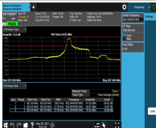
Band5-1.4MHz-QPSK-20407-6RB#0
