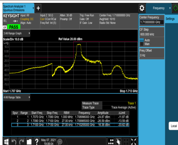
Band4-1.4MHz-16QAM-19957-6RB#0
