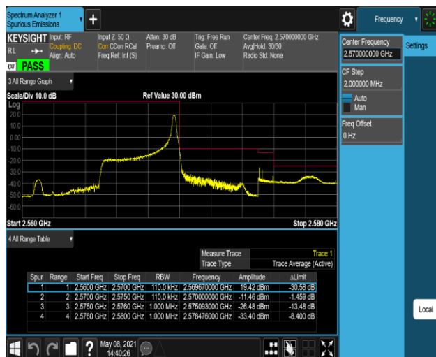
Band7-5MHz-16QAM-21425-1RB#24
