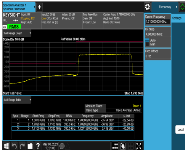
Band4-20MHz-16QAM-20300-1RB#99
