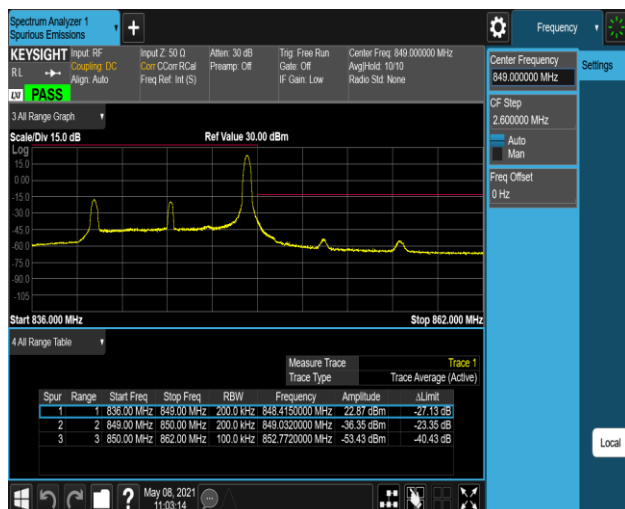
Band5-10MHz-QPSK-20600-1RB#49
