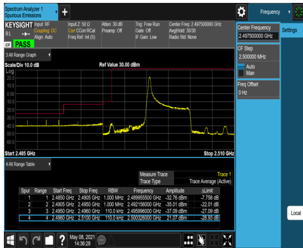
Band7-5MHz-16QAM-20775-25RB#0
