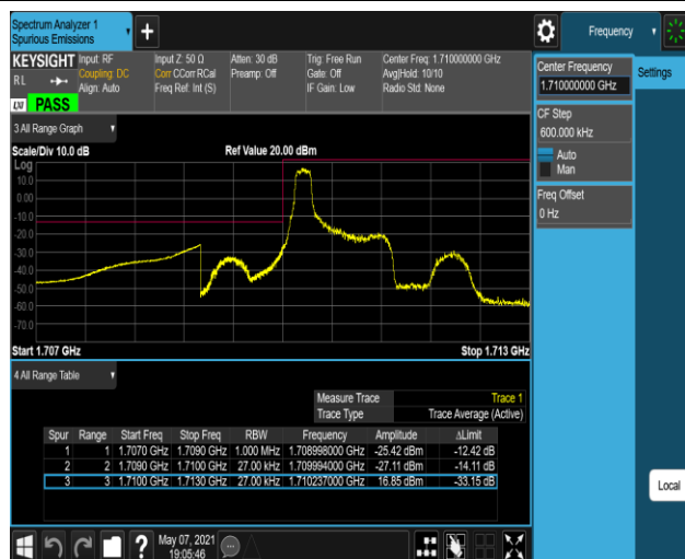
Band4-1.4MHz-QPSK-19957-6RB#0
