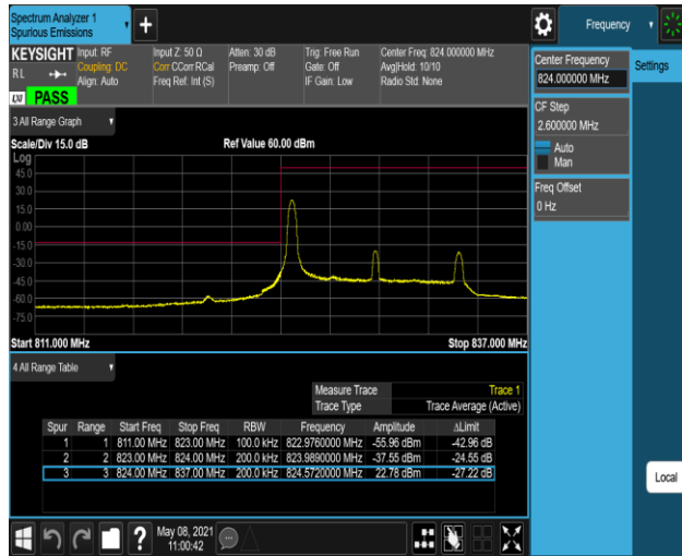
Band5-10MHz-QPSK-20450-50RB#0
