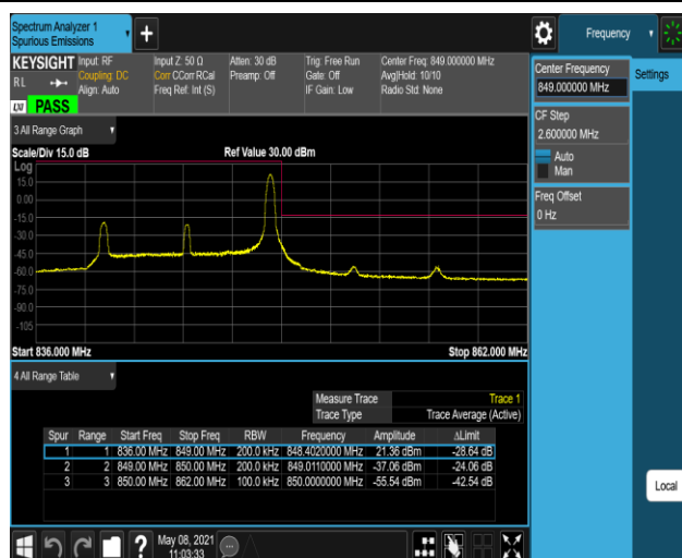
Band5-10MHz-16QAM-20600-1RB#49
