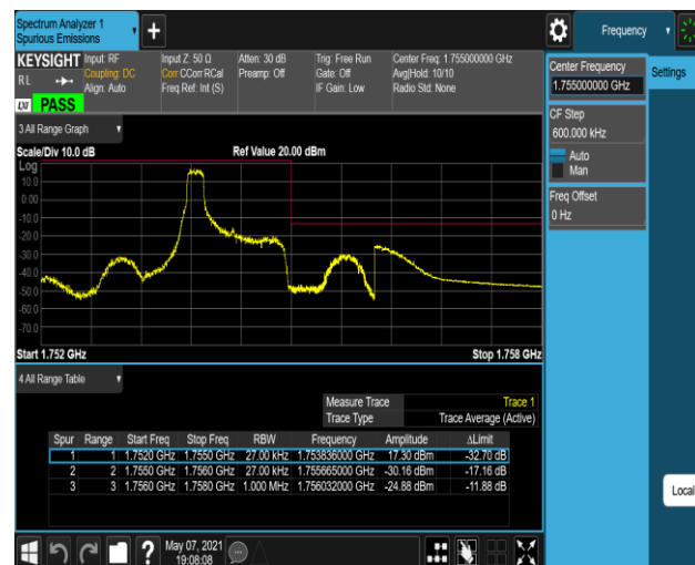
Band4-1.4MHz-16QAM-20393-6RB#0
