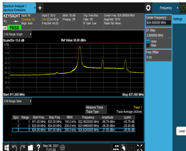
Band5-10MHz-16QAM-20450-50RB#0
