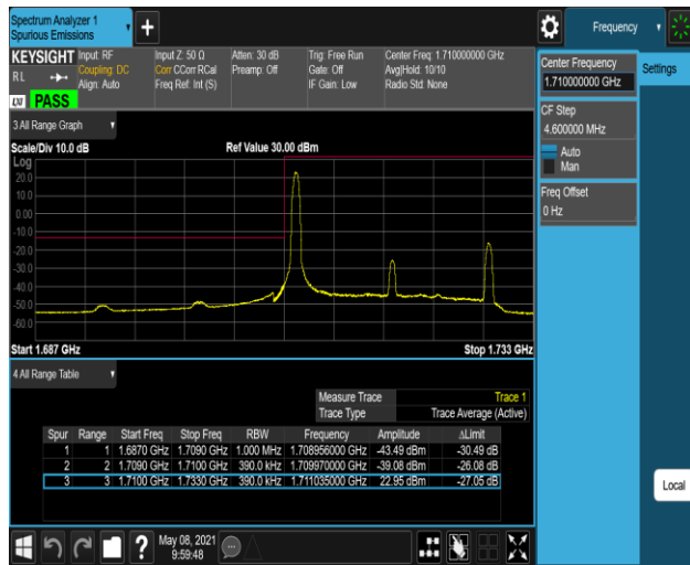
Band4-20MHz-16QAM-20050-100RB#0
