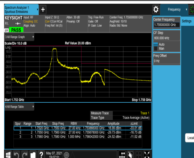
Band4-1.4MHz-QPSK-20393-6RB#0
