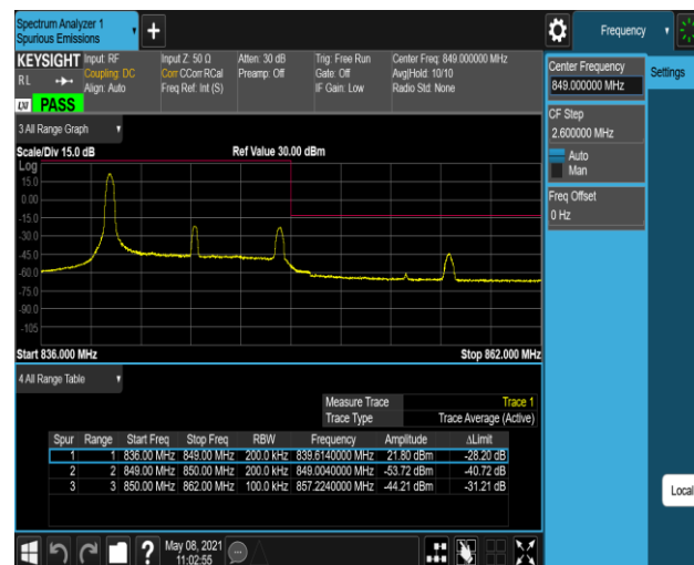
Band5-10MHz-16QAM-20600-50RB#0
