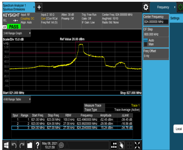
Band5-1.4MHz-16QAM-20407-6RB#0
