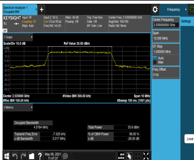
Band7-5MHz-16QAM-21100-25RB#0
