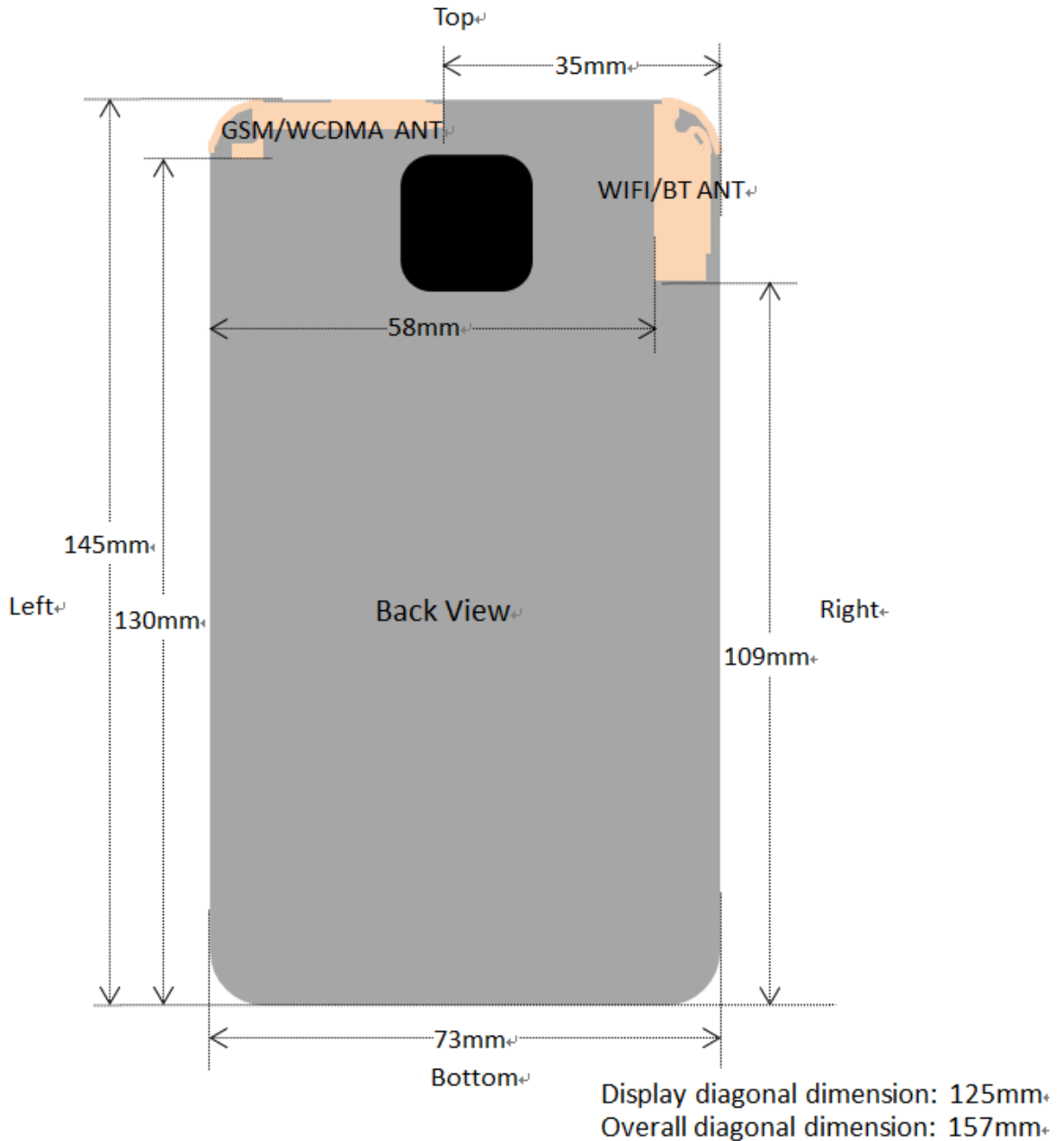
Fig.14.1 EUT Antenna Locations
