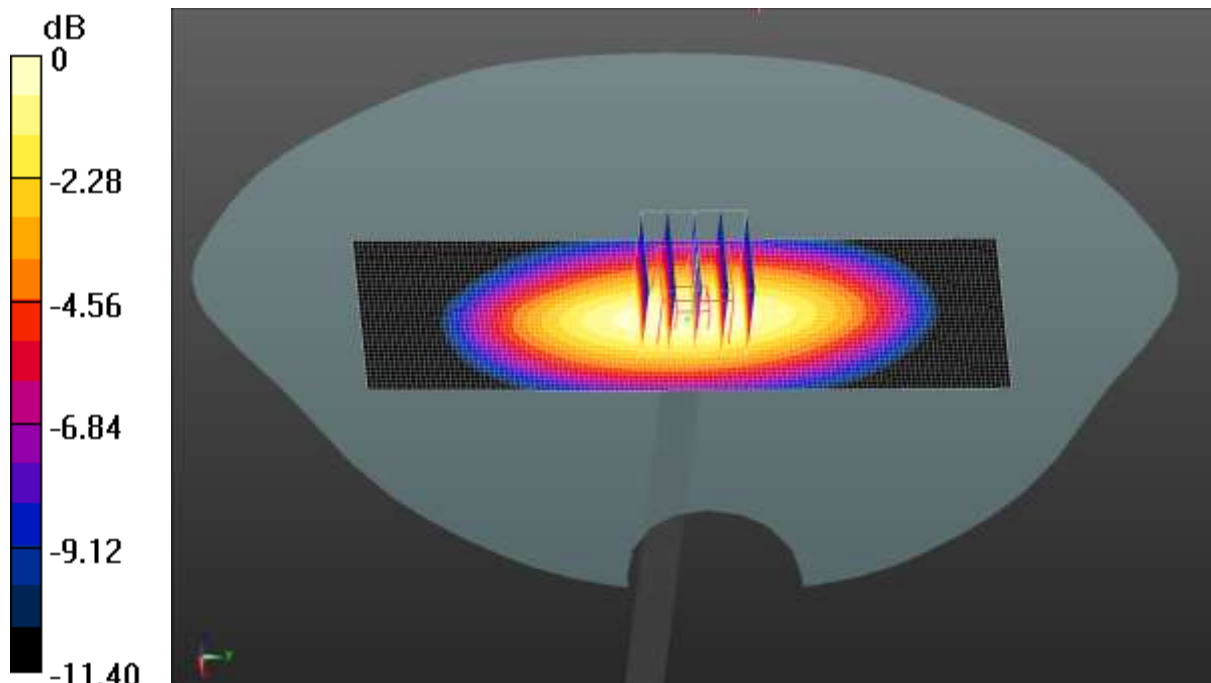
0 dB = 0.965 W/kg = -0.15 dBW/kg
