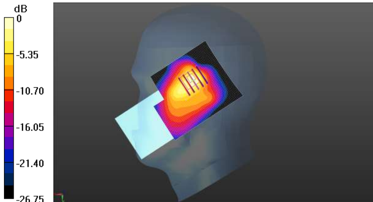
0 dB = 0.799 W/kg = -0.97 dBW/kg
