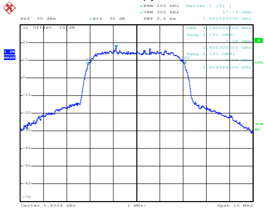
99% Occupy bandwidth
