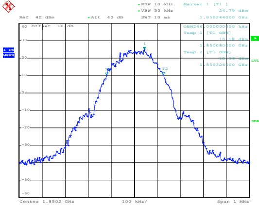
99% Occupy bandwidth
