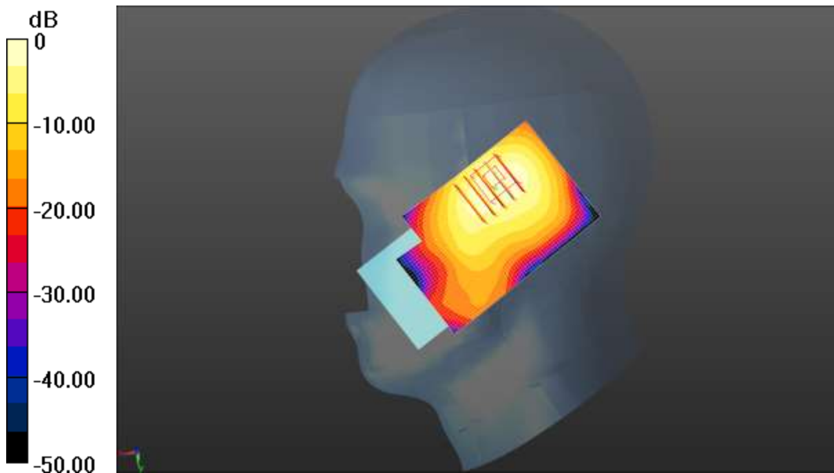
0 dB = 0.315 W/kg = -5.02 dBW/kg
