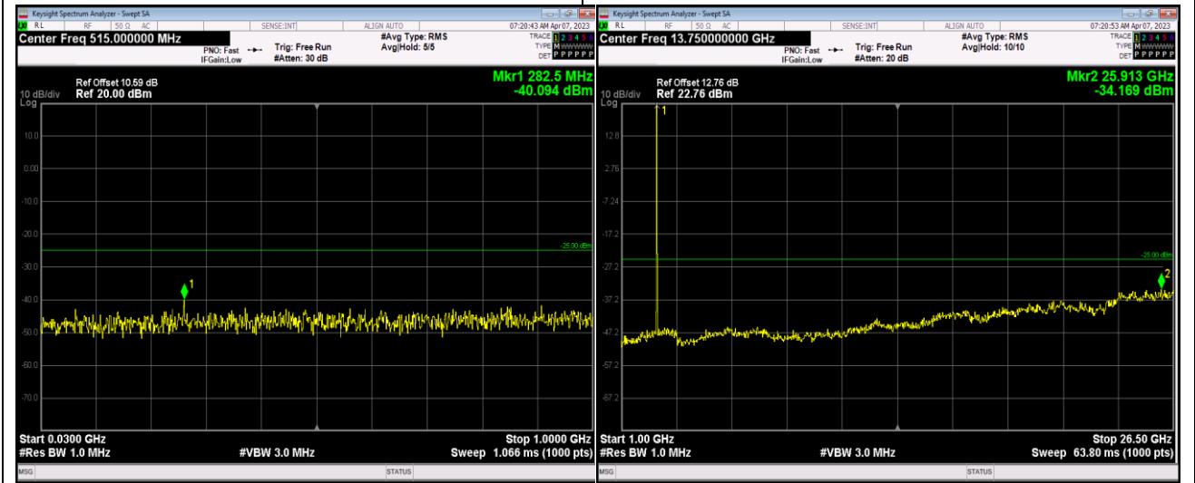
Band41-20MHz-16QAM-40140-1RB#0-Range1:30~1000MHz
