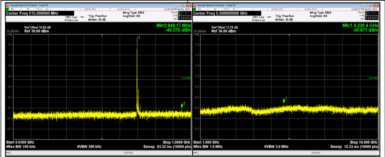
Band17-10MHz-64QAM-23780-1RB#0-Range1:30 ~1000MHz
