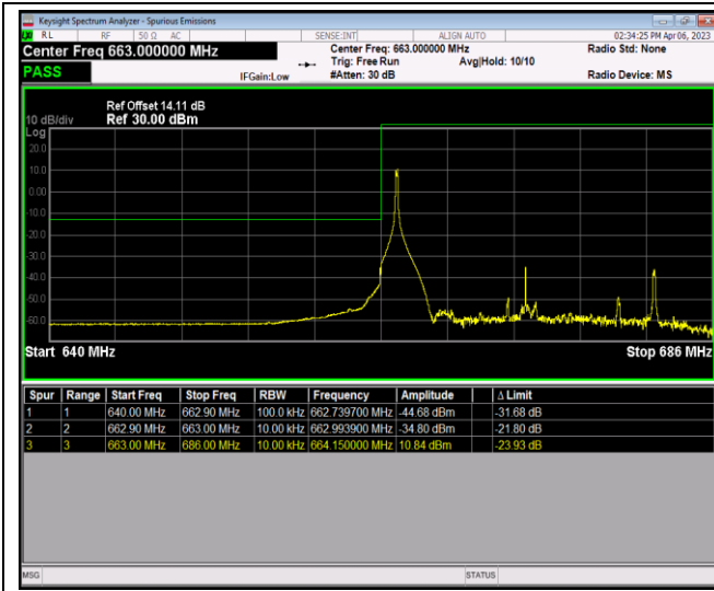
Band71-20MHz-64QAM-133222-100RB#0
