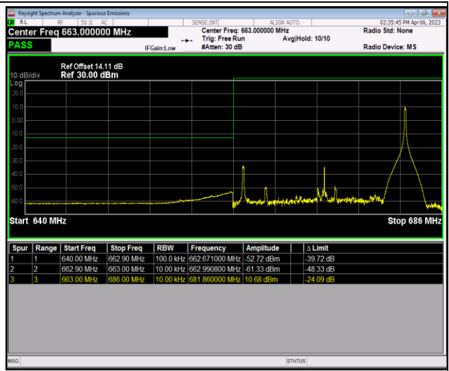
Band71-20MHz-64QAM-133372-1RB#0
