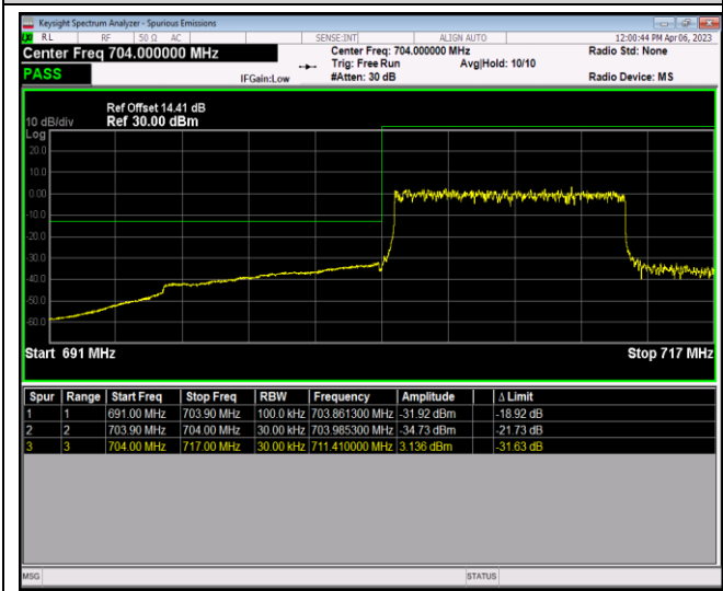
Band17-10MHz-QPSK-23800-1RB#49
