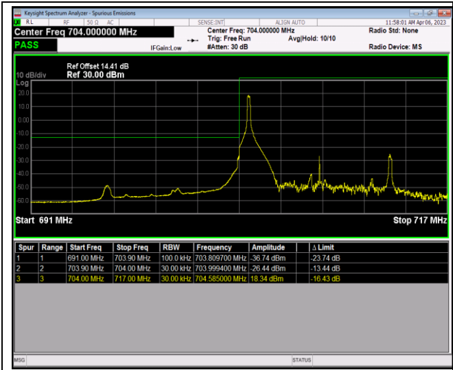
Band17-10MHz-QPSK-23780-50RB#0
