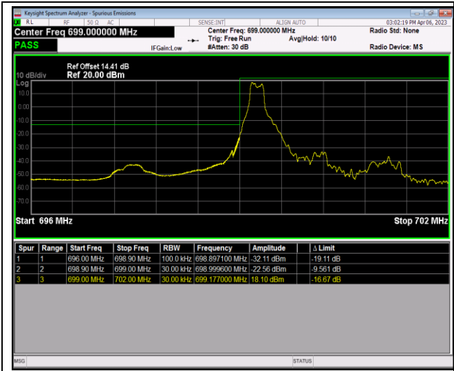
Band12-1.4MHz-QPSK-23017-6RB#0
