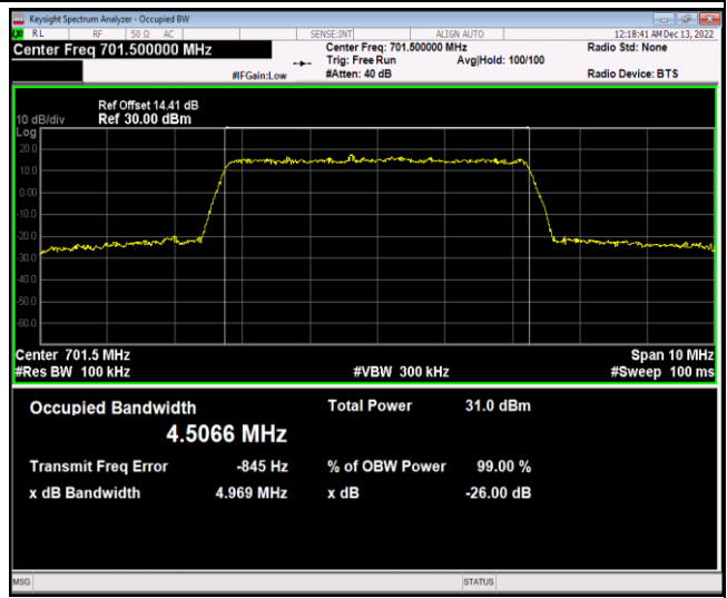
Band12-5MHz-16QAM-23155-25RB#0
