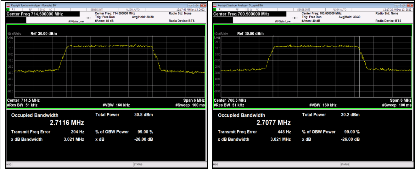
Band12-3MHz-16QAM-23095-15RB#0
