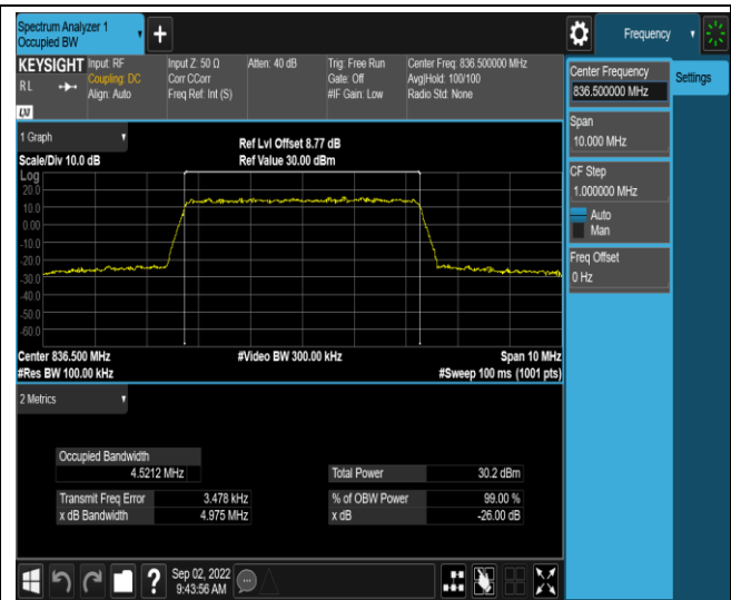
Band5-5MHz-16QAM-20425-25RB#0
