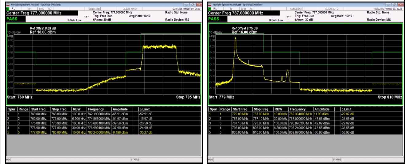
Band13-5MHz-16QAM-23255-1RB#24
