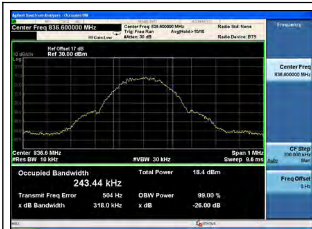
GSM 850 BW - Mid CH 836.6MHz
