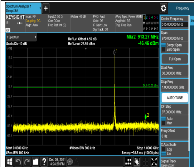
Band17-5MHz-QPSK-23755-1RB#0-Range1:30~1000MHz
