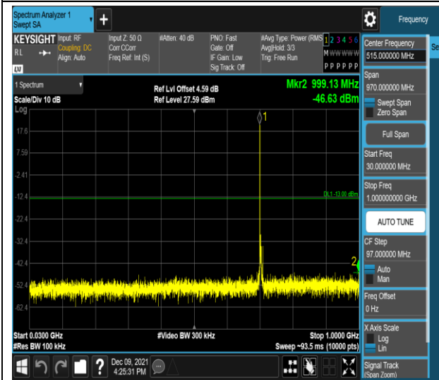
Band17-5MHz-QPSK-23755-1RB#0-Range1:30~1000MHz
