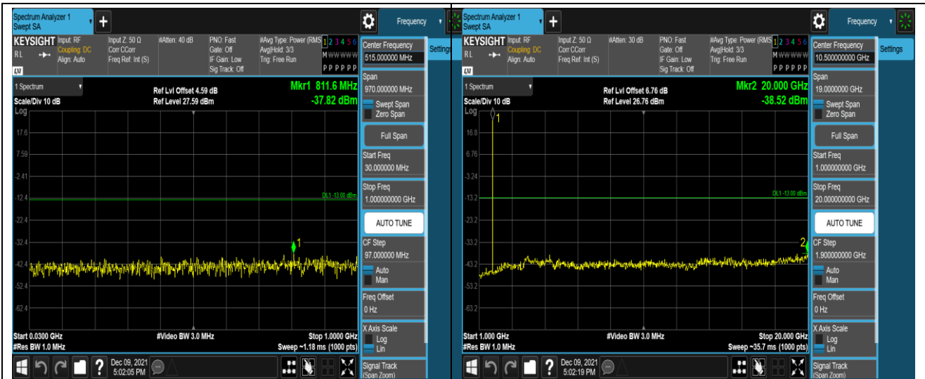
Band66-1.4MHz-QPSK-132665-1RB#0-Range1:30 ~1000MHz Band66-1.4MHz-QPSK-132665-1RB#0-Range2:1000 ~20000MHz
