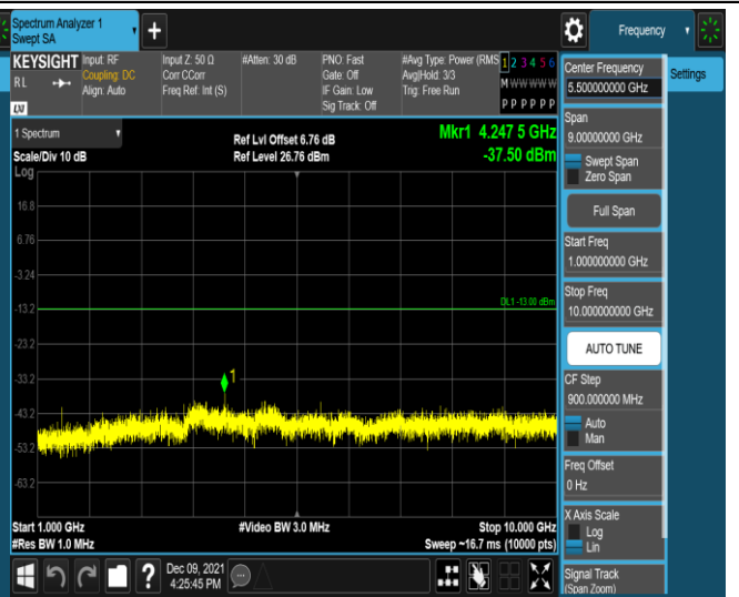
Band17-5MHz-QPSK-23755-1RB#0-Range2:1000~10000MHz
