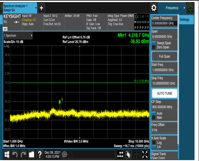
Band12-10MHz-QPSK-23095-1RB#0-Range2:1000~10000MHz
