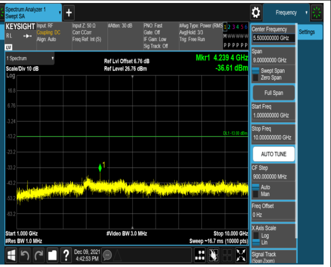
Band17-10MHz-16QAM-23790-1RB#0-Range2:1000~ 10000MHz
