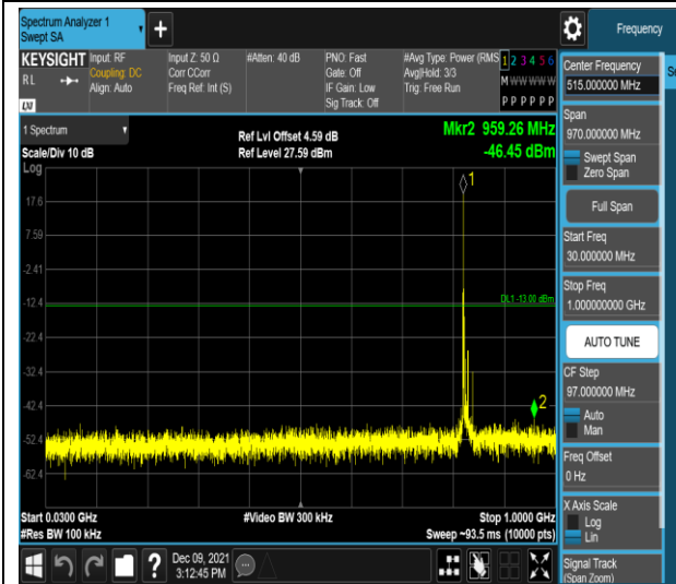
Band5-10MHz-16QAM-20450-1RB#0-Range1:30~1000MHz
