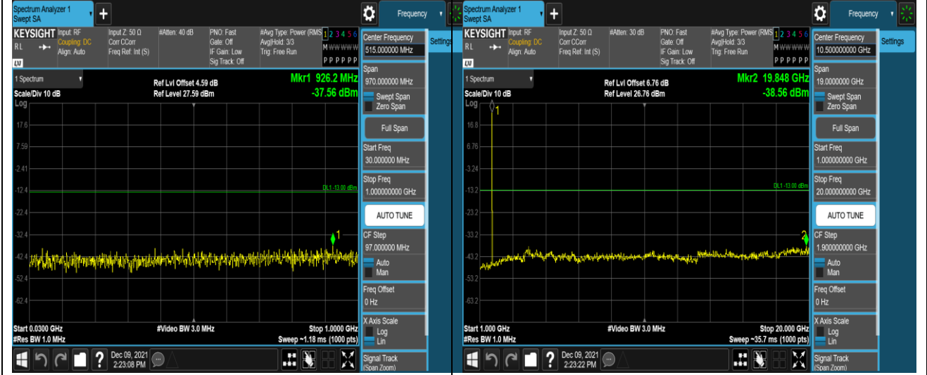
Band4-20MHz-QPSK-20050-1RB#0-Range1:30~1000MHz
