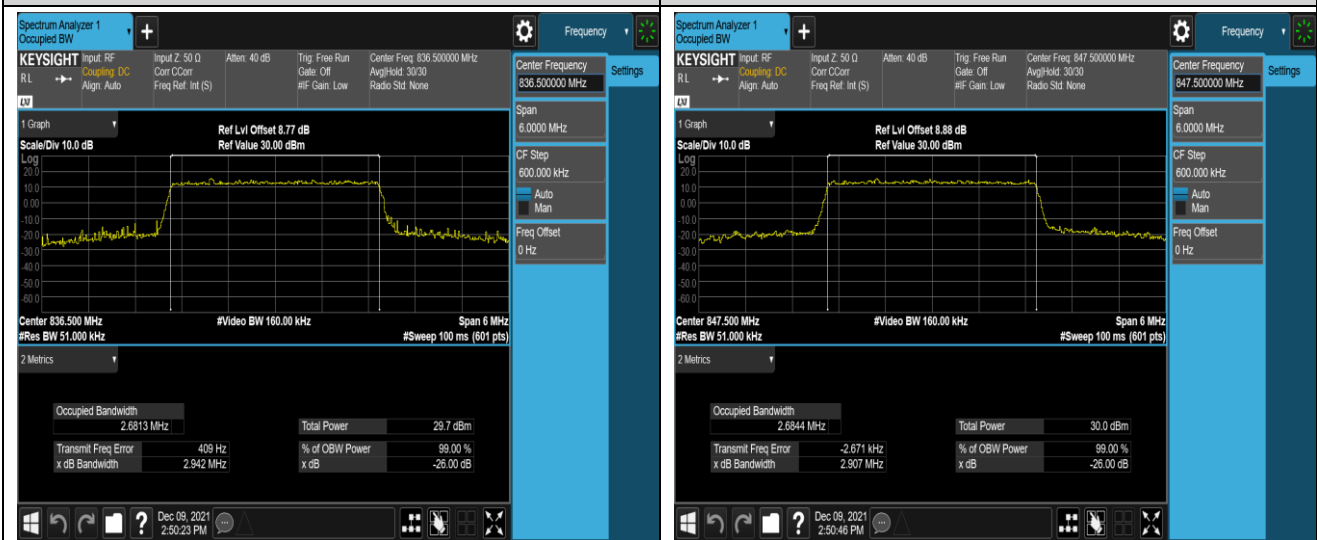
Band5-3MHz-16QAM-20525-15RB#0
