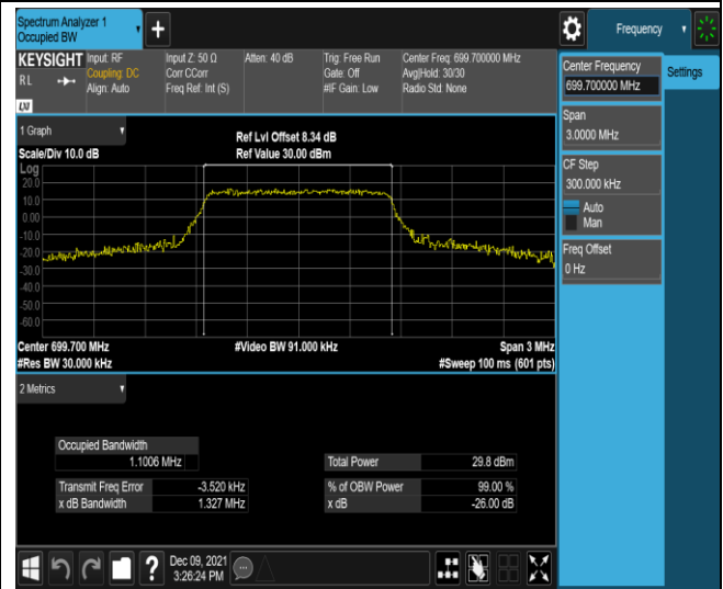
Band12-1.4MHz-16QAM-23017-6RB#0
