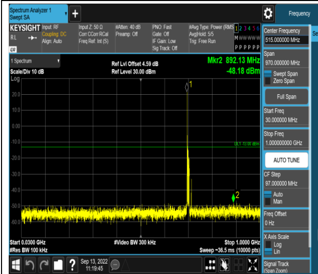
Band12-10MHz-QPSK-23130-1RB#0-Range1:30~1000MHz
