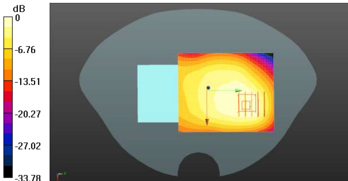
0 dB = 0.210 W/kg = -6.78 dBW/kg
