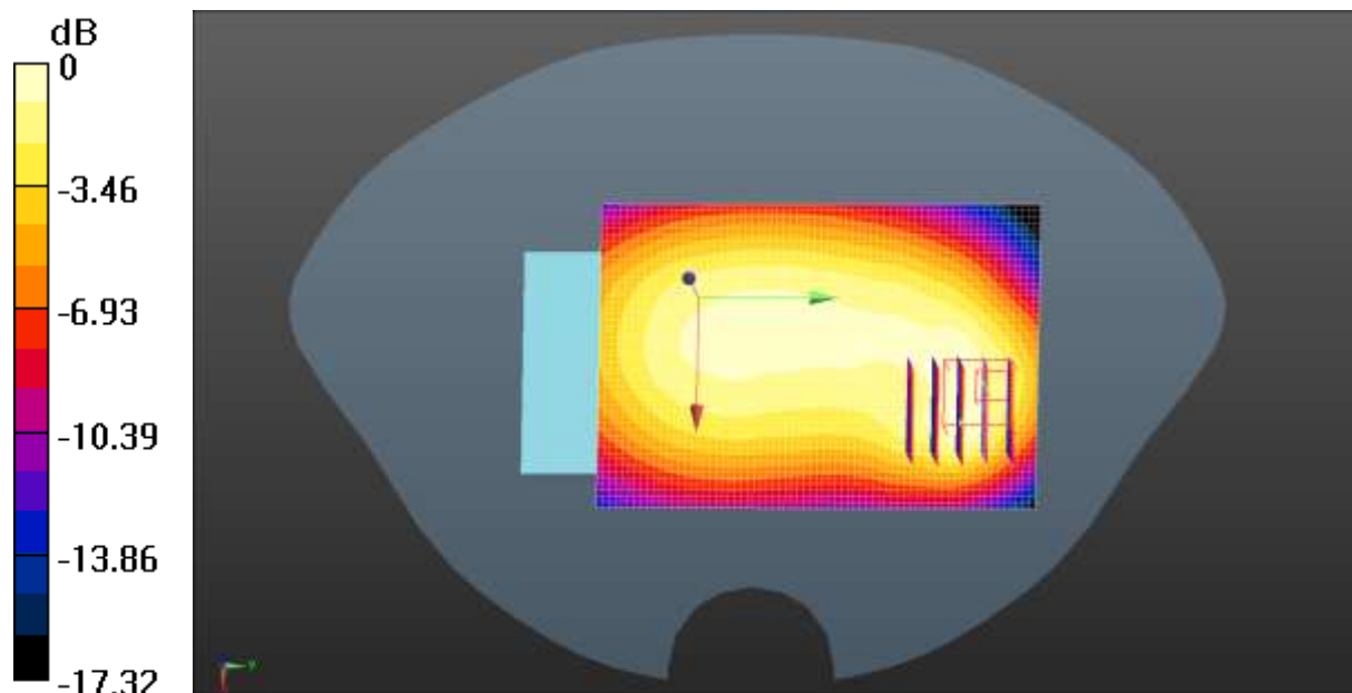
0 dB = 0.413 W/kg = -3.84 dBW/kg
