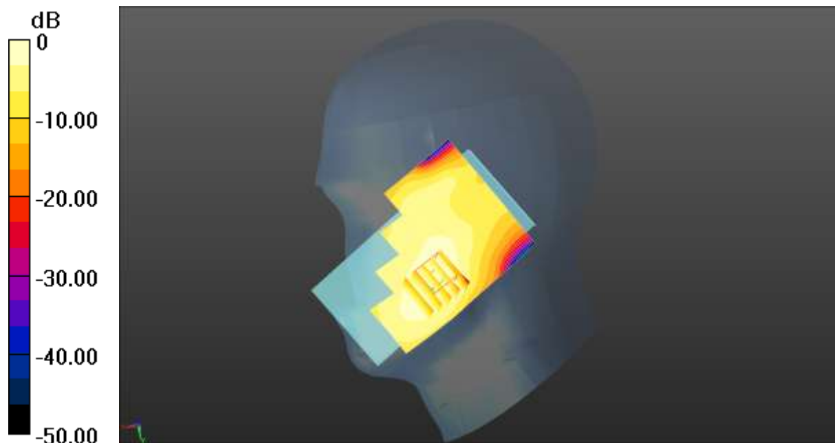
0 dB = 0.122 W/kg = -9.14 dBW/kg
