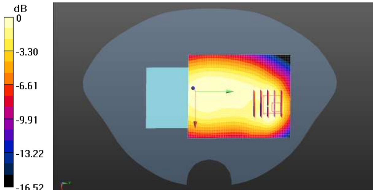
0 dB = 0.452 W/kg = -3.45 dBW/kg
