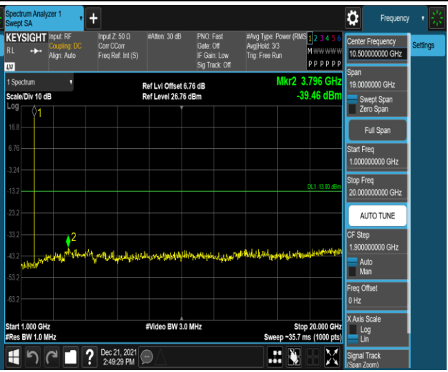
Band66-1.4MHz-16QAM-131979-1RB#0-Range2:100 0~20000MHz
