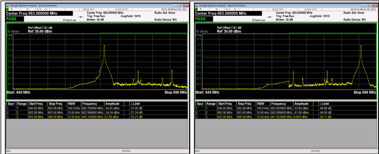
Band71-20MHz-16QAM-133222-100RB#0
