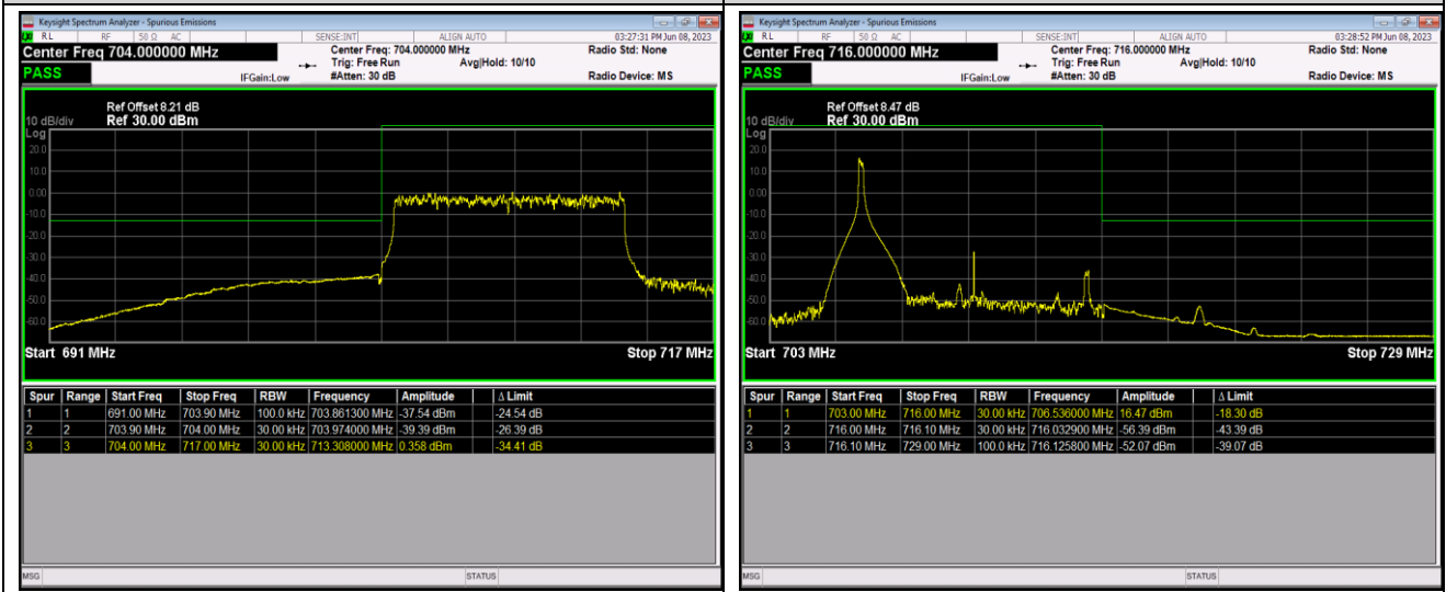
Band17-10MHz-16QAM-23800-1RB#49
