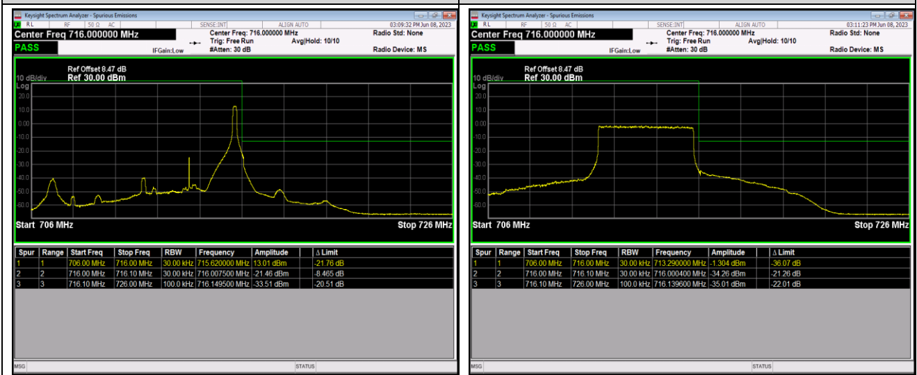
Band17-10MHz-QPSK-23780-1RB#0
