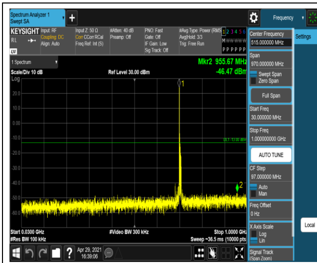
Band17-5MHz-QPSK-23755-1RB#0-Range1:30~1000MHz
