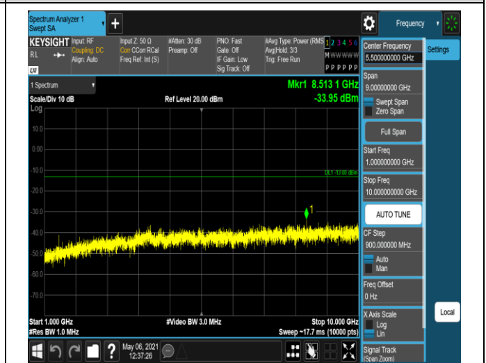
Band17-5MHz-QPSK-23790-1RB#0-Range2:1000~10000MHz
