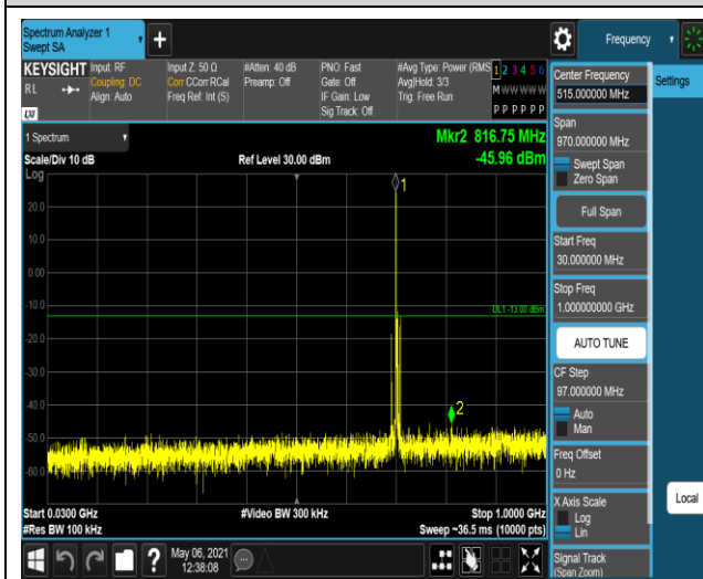
Band17-5MHz-QPSK-23755-1RB#0-Range1:30~1000MHz
