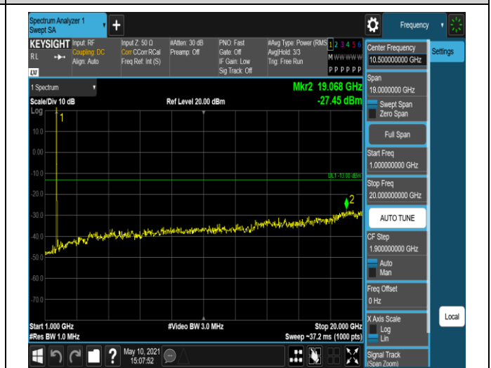
Band66-20MHz-16QAM-132072-1RB#0-Range2:1000~20000MHz
