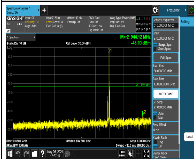
Band17-5MHz-QPSK-23790-1RB#0-Range1:30~1000MHz
