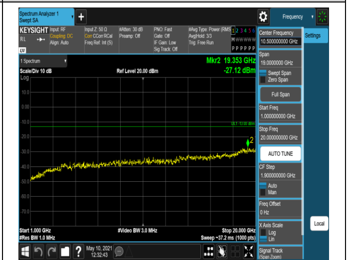
Band66-1.4MHz-16QAM-132322-1RB#0-Range2:1000 ~20000MHz
