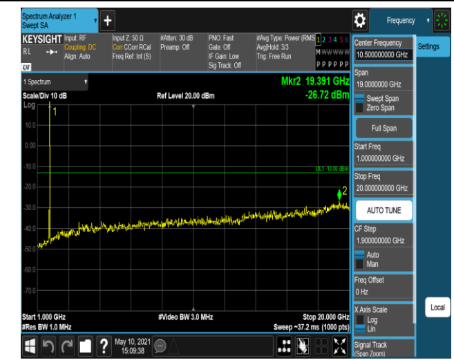
Band66-20MHz-16QAM-132572-1RB#0-Range2:1000~ 20000MHz
