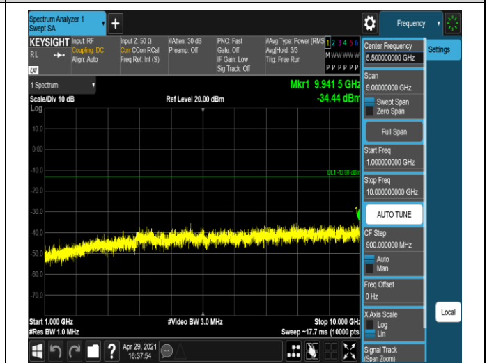
Band12-10MHz-QPSK-23130-1RB#0-Range2:1000~10000MHz
