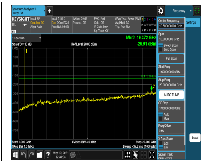
Band66-1.4MHz-16QAM-131979-1RB#0-Range2:1000 ~20000MHz
