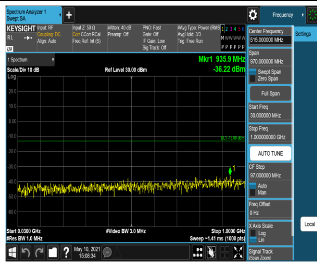
Band66-20MHz-16QAM-132572-1RB#0-Range1:30 ~1000MHz
