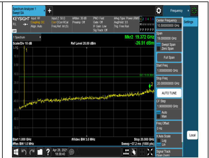
Band4-20MHz-16QAM-20300-1RB#0-Range2:1000~20000MHz
