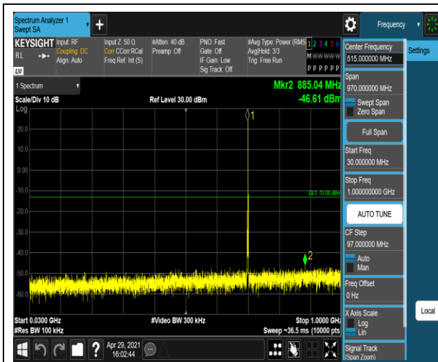
Band12-1.4MHz-QPSK-23173-1RB#0-Range1:30~1000MHz
