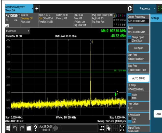
Band12-1.4MHz-16QAM-23017-1RB#0-Range1:30~1000MHz
