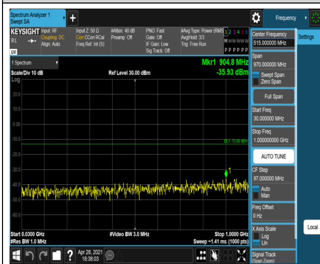
Band4-20MHz-QPSK-20715-1RB#0-Range1:30~1000MHz
