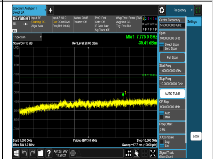
Band5-1.4MHz-QPSK-20407-1RB#0-Range2:1000~10000MHz
