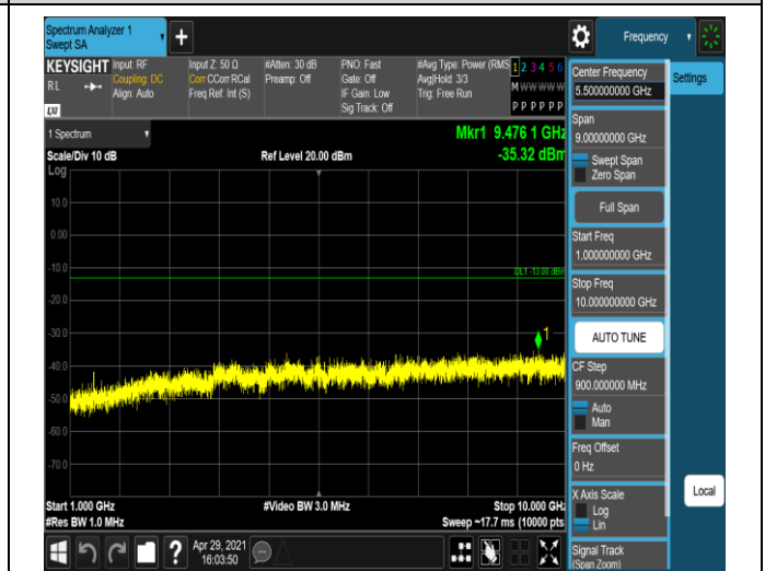
Band12-1.4MHz-16QAM-23017-1RB#0-Range2:1000~10000MHz
