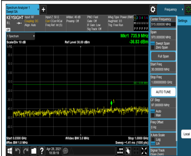
Band5-1.4MHz-QPSK-20407-1RB#0-Range1:30~1000MHz
