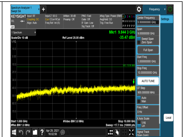
Band12-1.4MHz-QPSK-23173-1RB#0-Range2:1000~10000MHz
