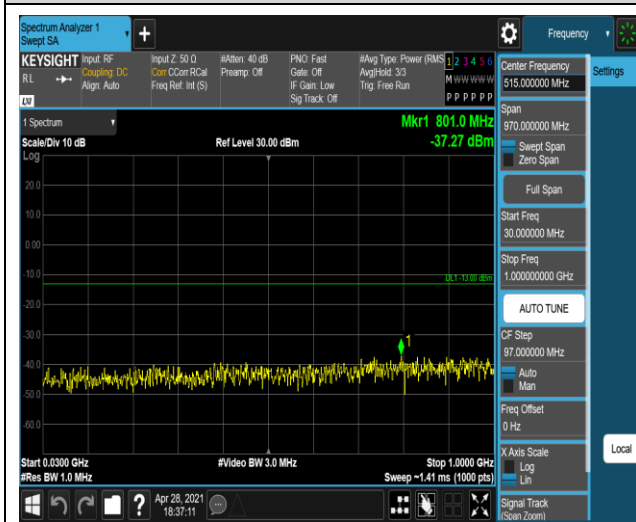
Band4-20MHz-QPSK-20175-1RB#0-Range1:30~1000MHz
