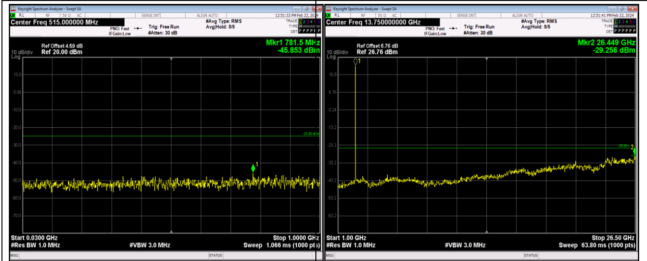
Band7-20MHz-QPSK-21100-1RB#0-Range1:30~1000MHz
