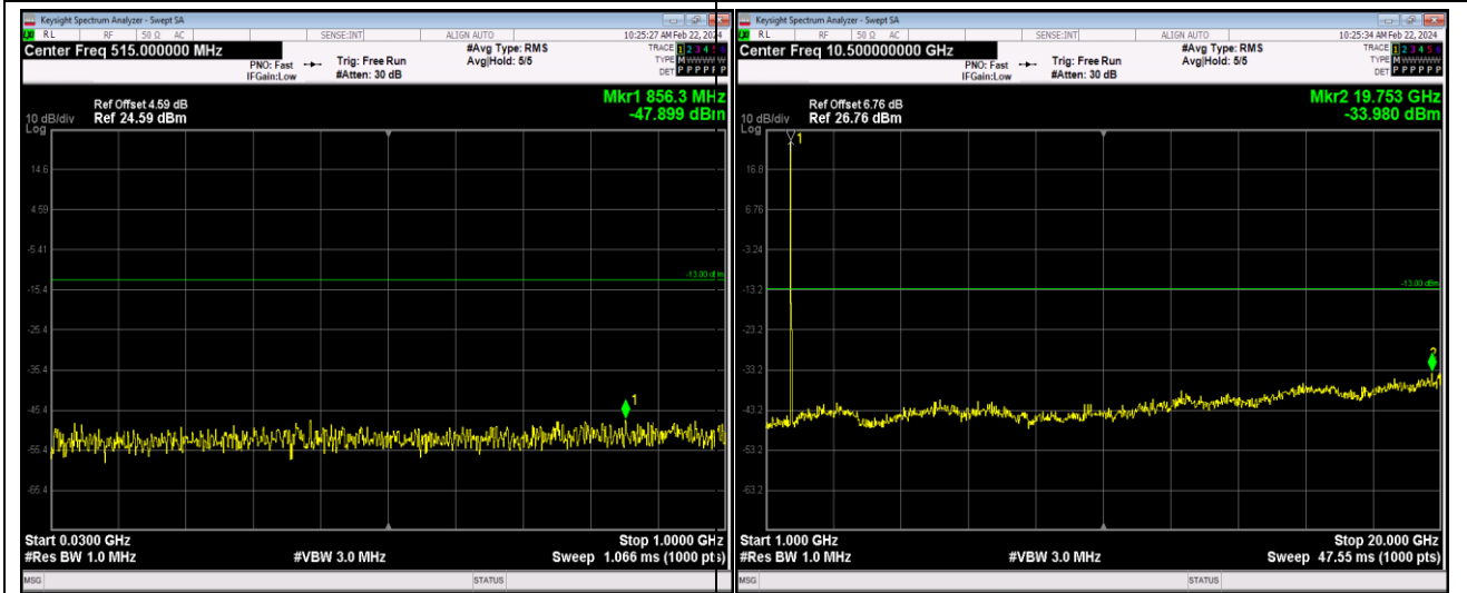
Band4-20MHz-64QAM-20175-1RB#0-Range1:30~1000MHz
