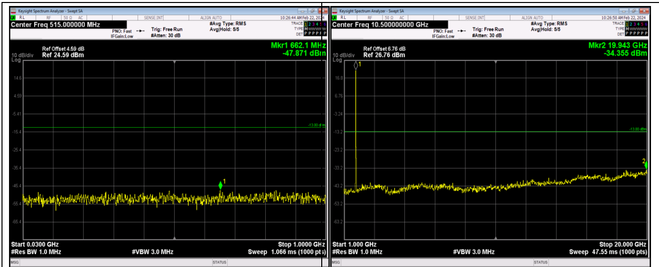
Band4-20MHz-64QAM-20050-1RB#0-Range1:30~1000MHz
