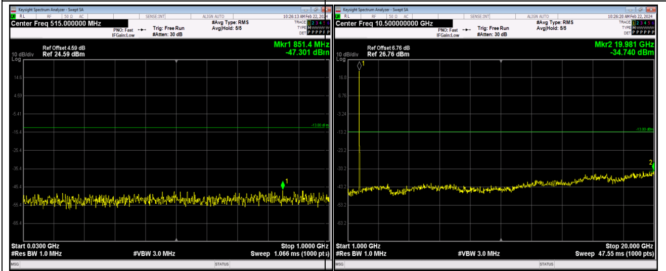
Band4-20MHz-64QAM-20175-1RB#0-Range1:30~1000MHz
