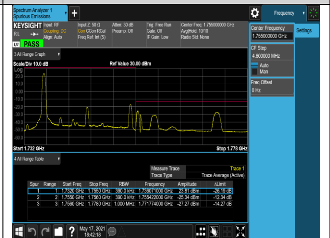
Band4-20MHz-QPSK-20300-100RB#0
