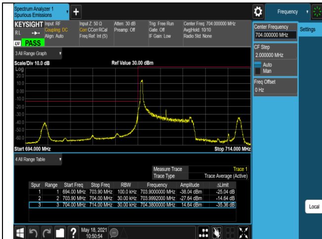
Band17-5MHz-16QAM-23755-25RB#0
