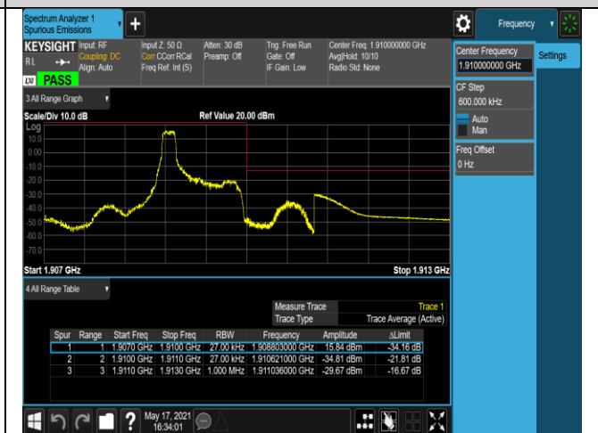
Band2-1.4MHz-16QAM-19193-6RB#0
